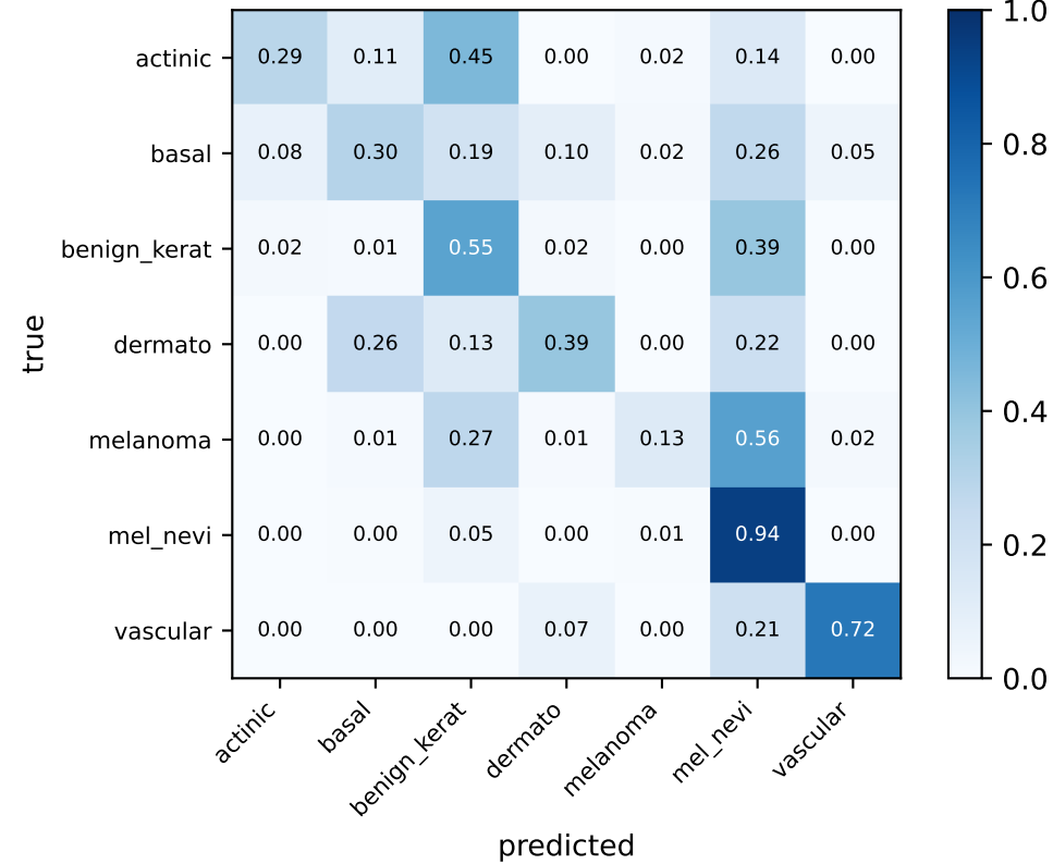
FedAvg (seed 42) — row-normalised
