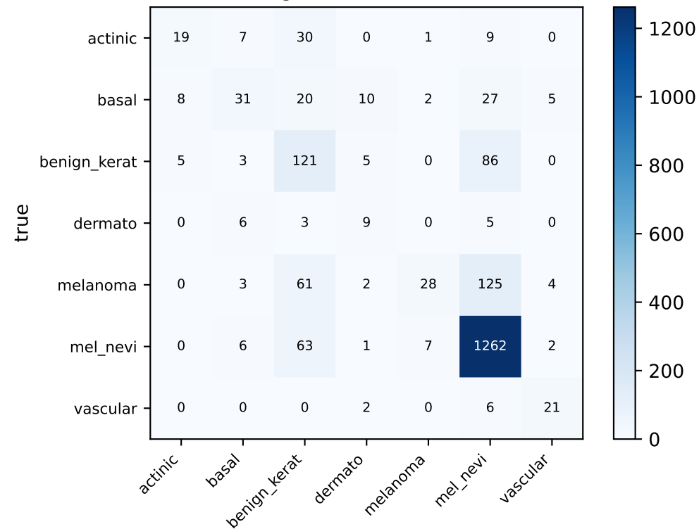
FedAvg (seed 42) — counts
