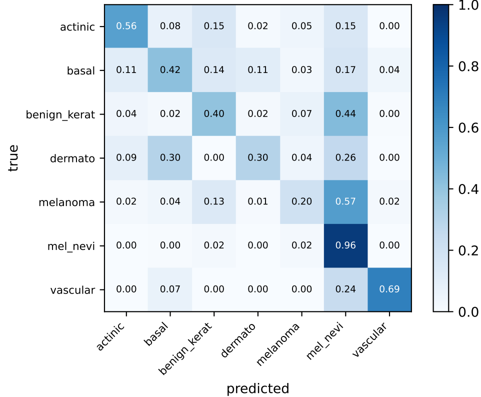
FedProx (seed 42) — row-normalised
