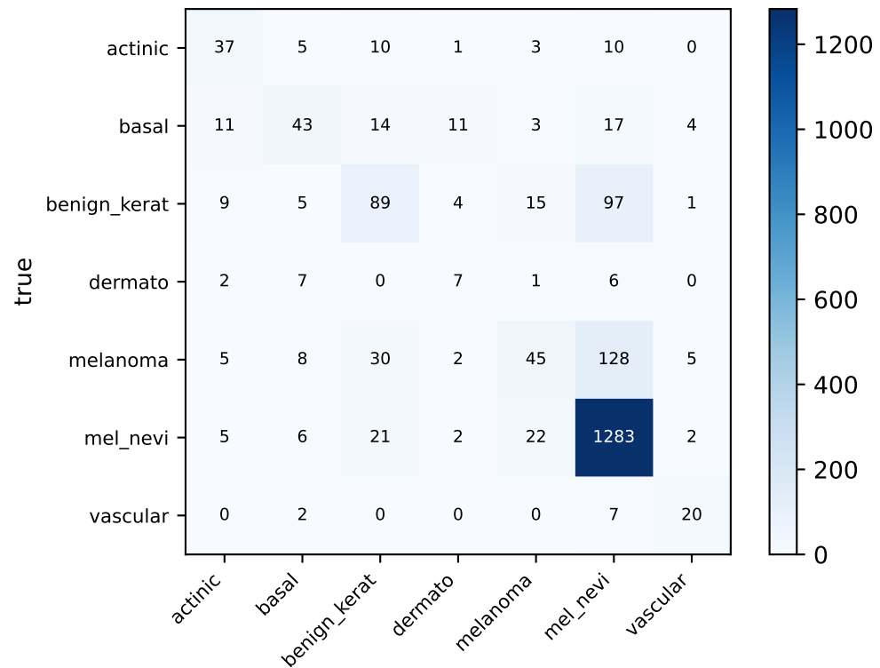
FedProx (seed 42) — counts
