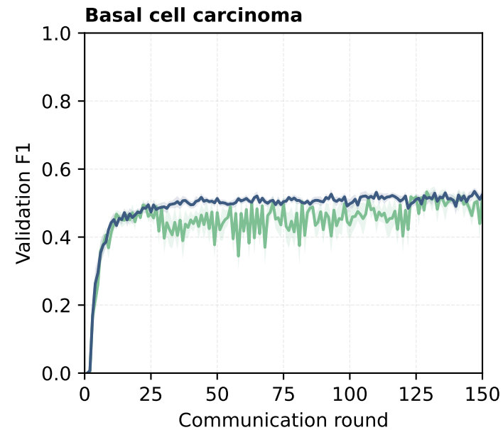
Per-class validation F1 over rounds (Flower runtime, n = 10 paired seeds, mean \pm SEM)
