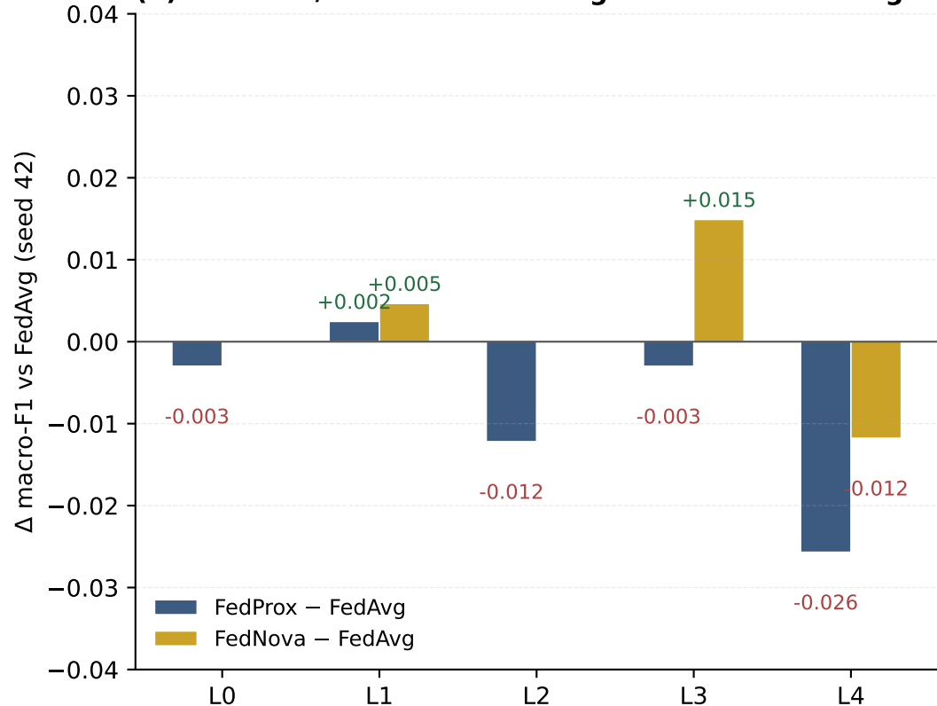
(b) FedProx / FedNova advantage relative to FedAvg
