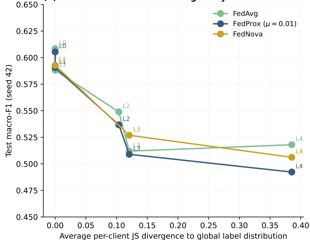
(a) Macro-F1 across the heterogeneity ladder
