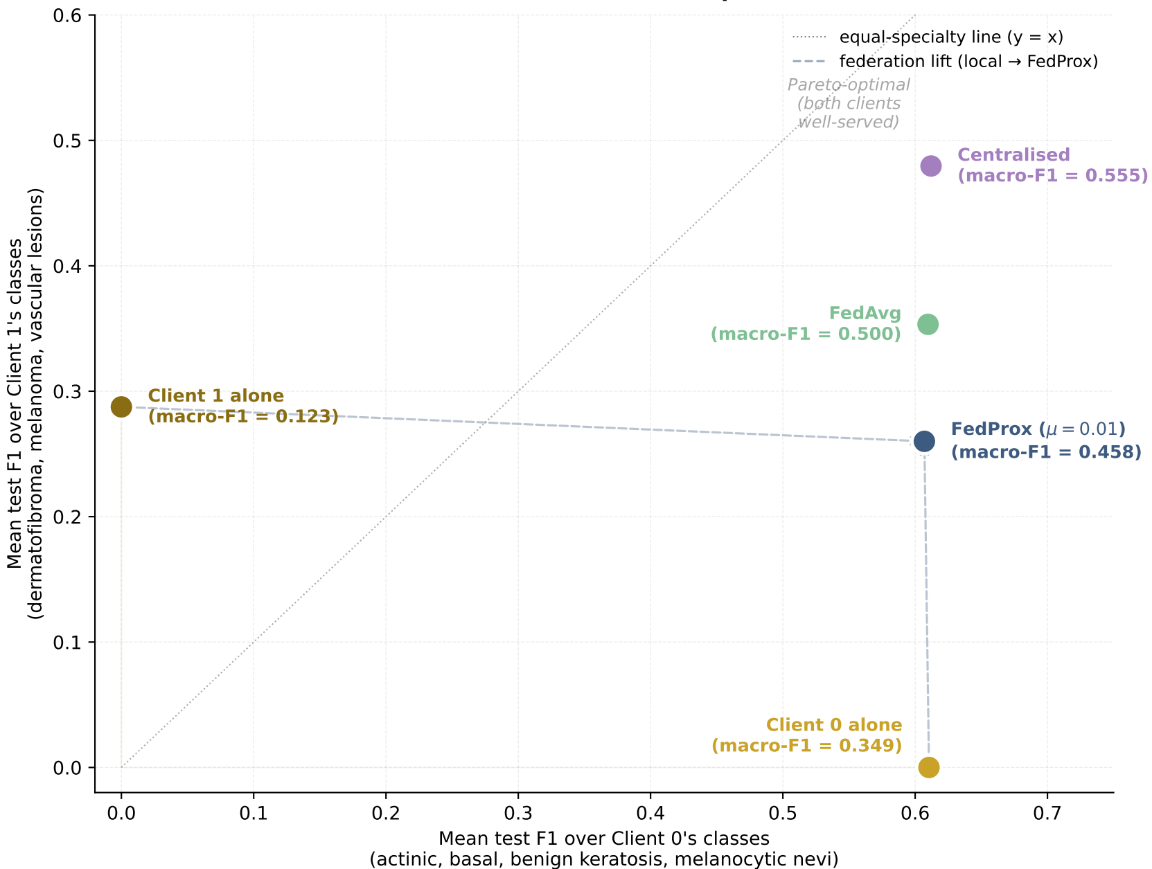
The federation Pareto frontier on the 2-client 90/10 partition (seed 42)
