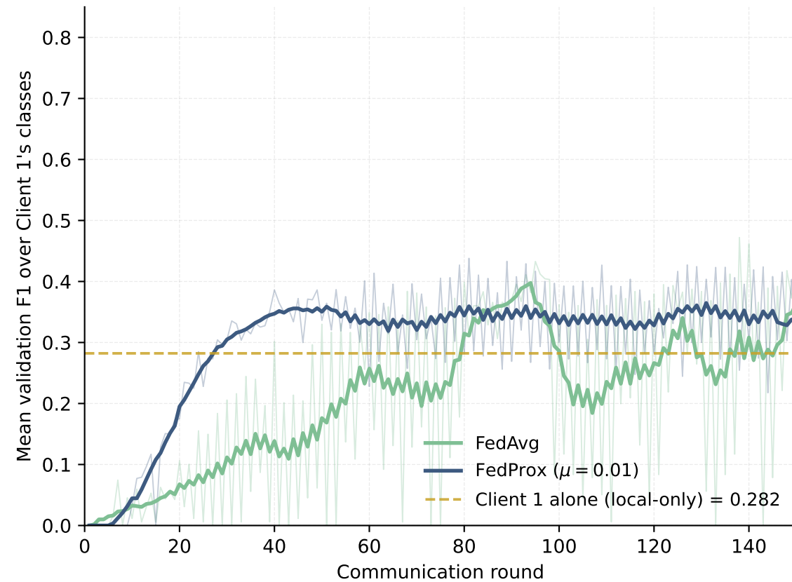
(b) Client 1's specialty (rare) — dermatofibroma, melanoma, vascular
