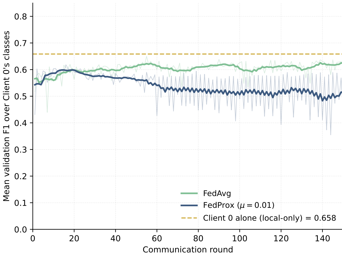
(a) Client 0's specialty — actinic, basal, benign keratosis, nevi
