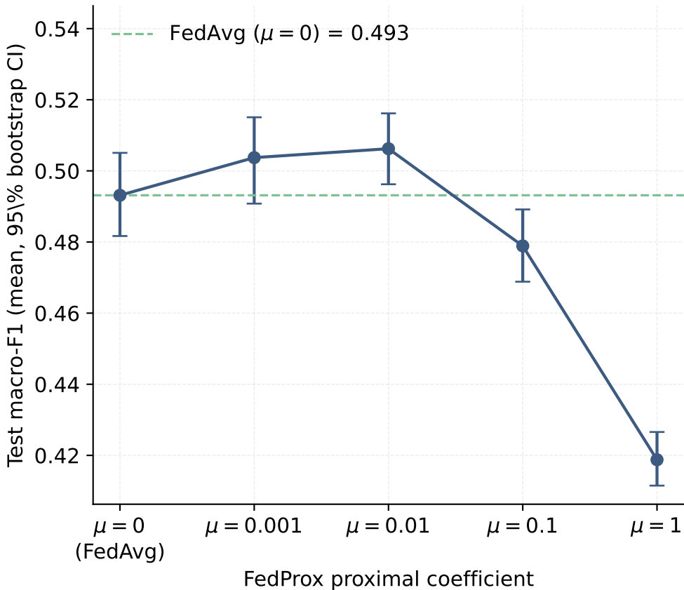
(a) Final test macro-F1
