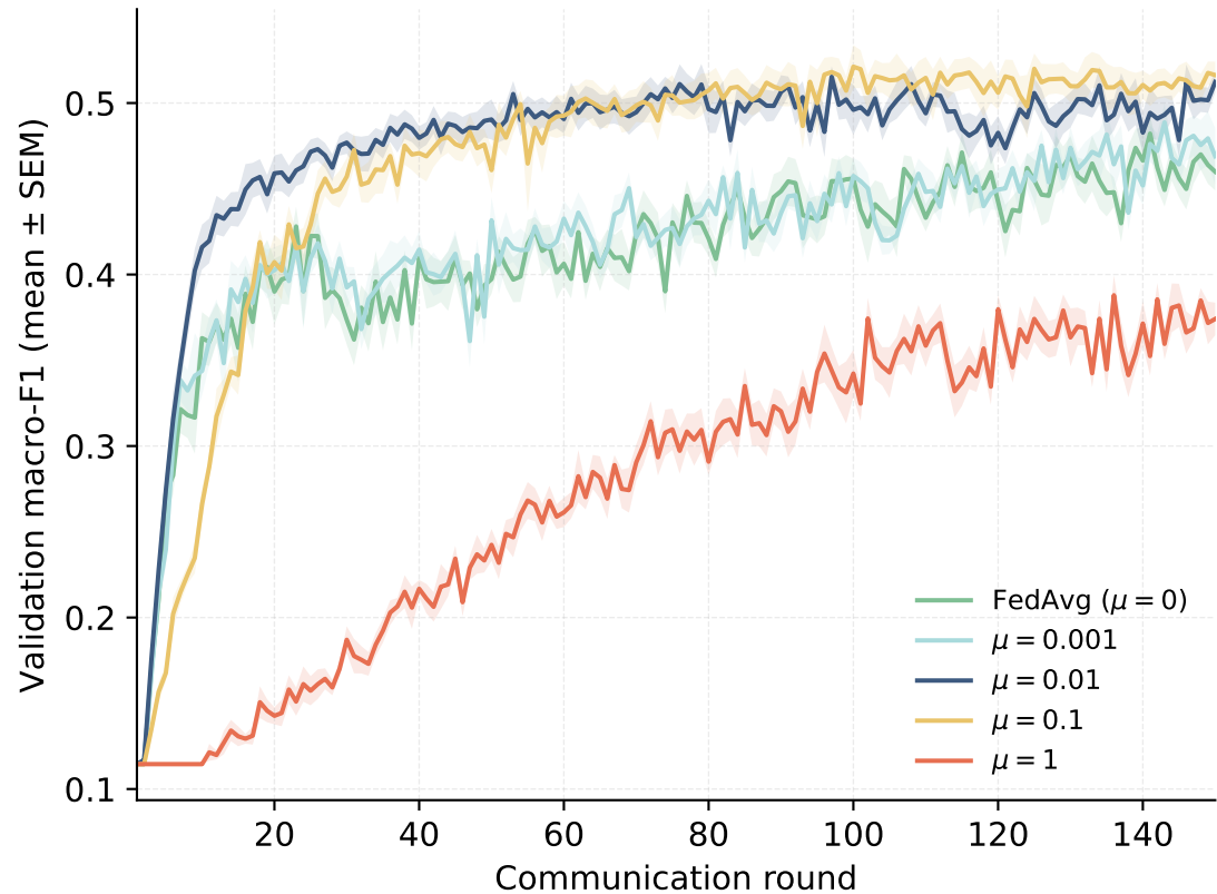
(b) Validation trajectory by \mu
