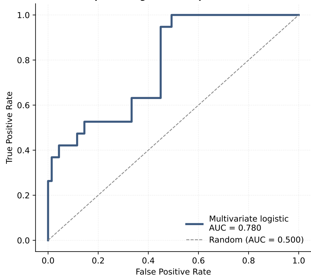
(a) ROC for predicting final collapse from round-20 features
