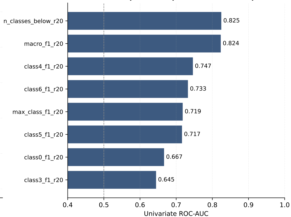
(b) Per-feature predictive power for final collapse
