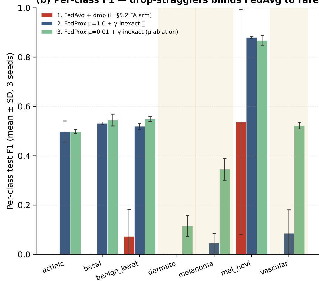
(b) Per-class F1 — drop-stragglers blinds FedAvg to rare classes
