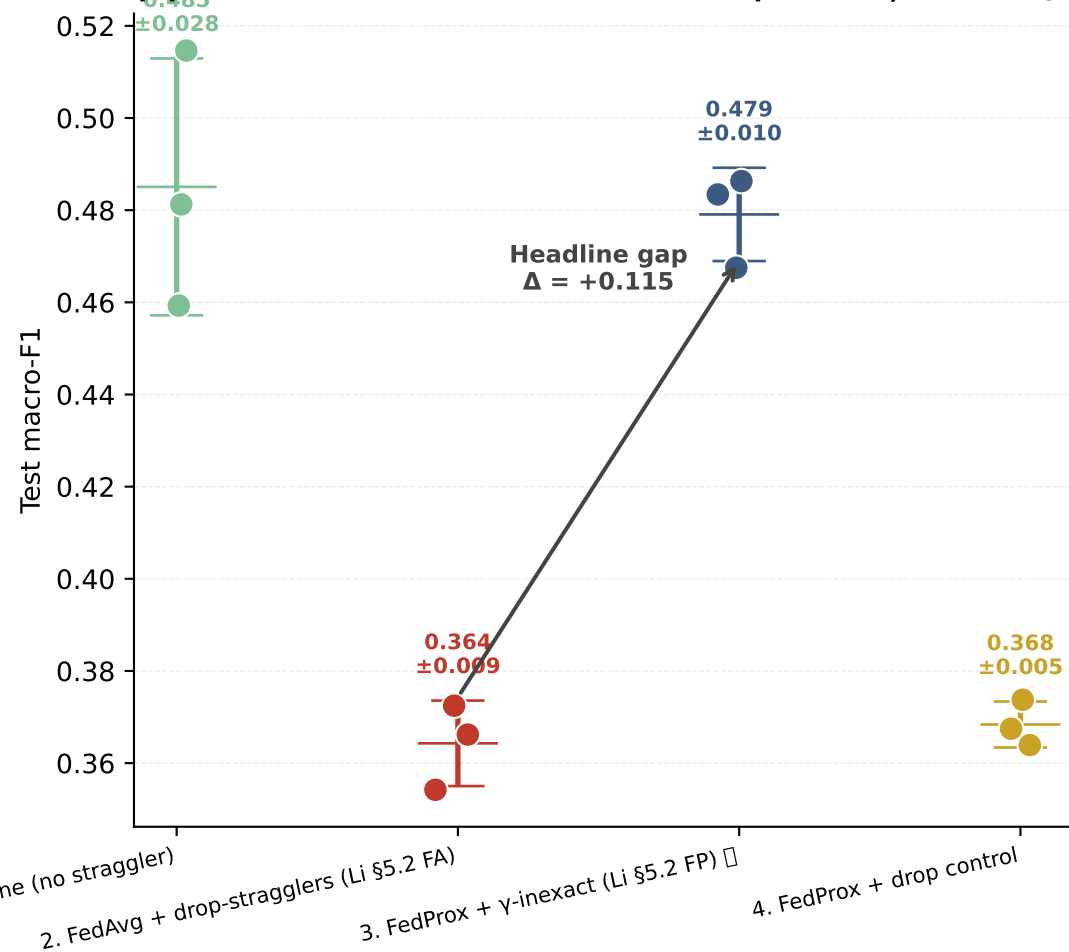
(a) Macro-F1 across the 4 conditions (3 seeds; Li 2020 §5.2)
