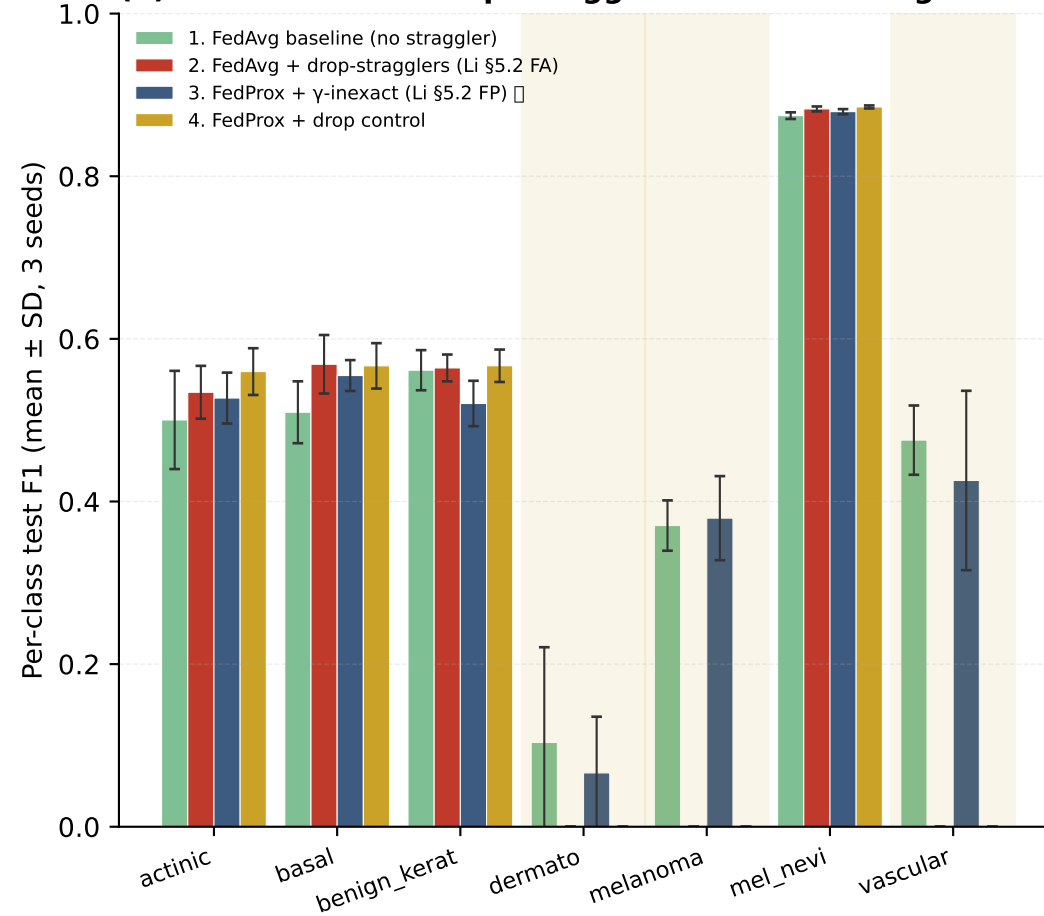
(b) Per-class F1 — drop-stragglers makes FedAvg blind to rare classes (shaded)
