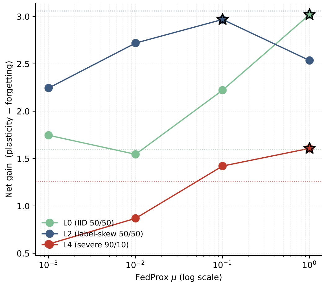
(a) Plasticity-forgetting Pareto cloud — colour = partition, marker = \mu (b) Net-gain Pareto curves — star marks \mu^* ; dotted = FedAvg baseline
