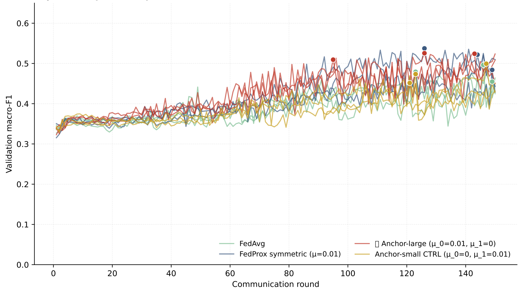
Asymmetric per-client \mu on L4 — validation macro-F1 (3 seeds, Yao 2024 ablation)
