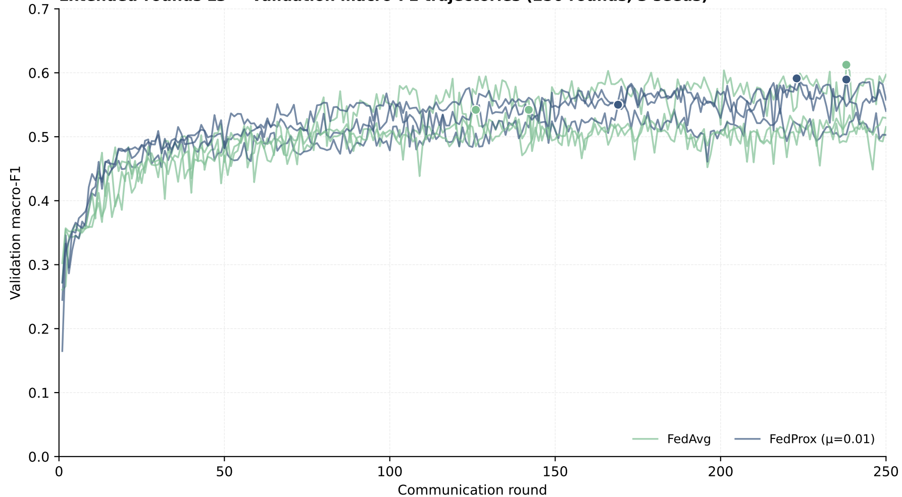
Extended-rounds L3 — validation macro-F1 trajectories (250 rounds, 3 seeds)
