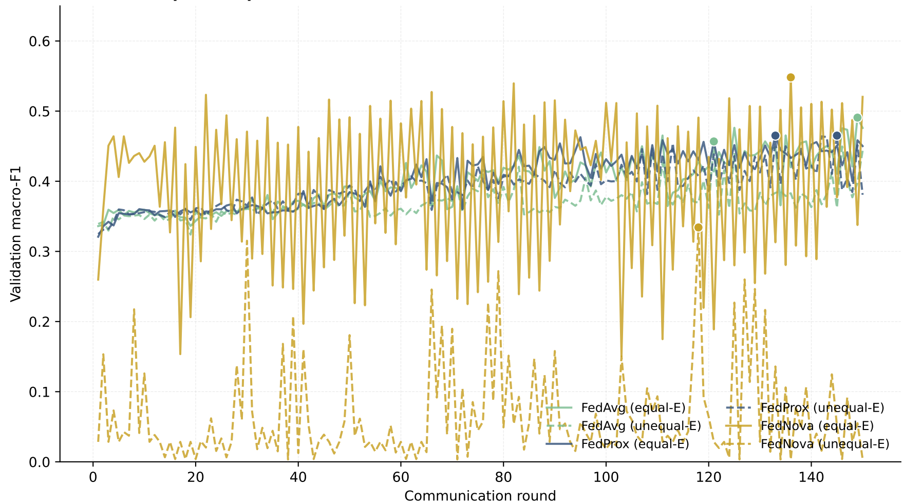
FedNova × equal/unequal-E at L4 — validation macro-F1 (seed 42)
