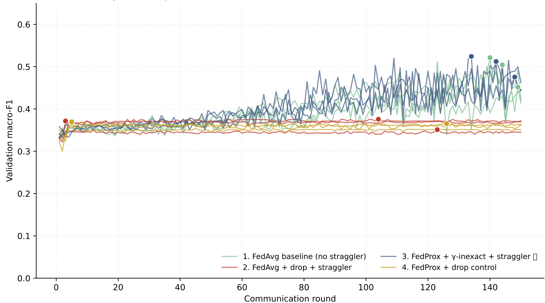
Li 2020 §5.2 asymmetric protocol on L4 — validation macro-F1 (3 seeds)
