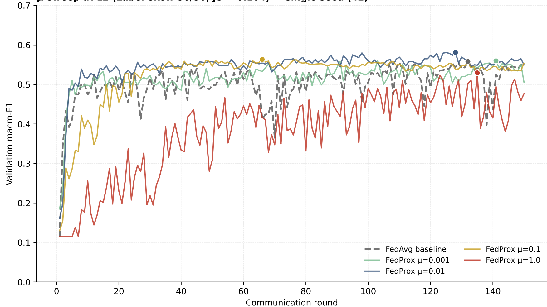
\mu -sweep at L2 (Label-skew 50/50, JS = 0.104) — single seed (42)
