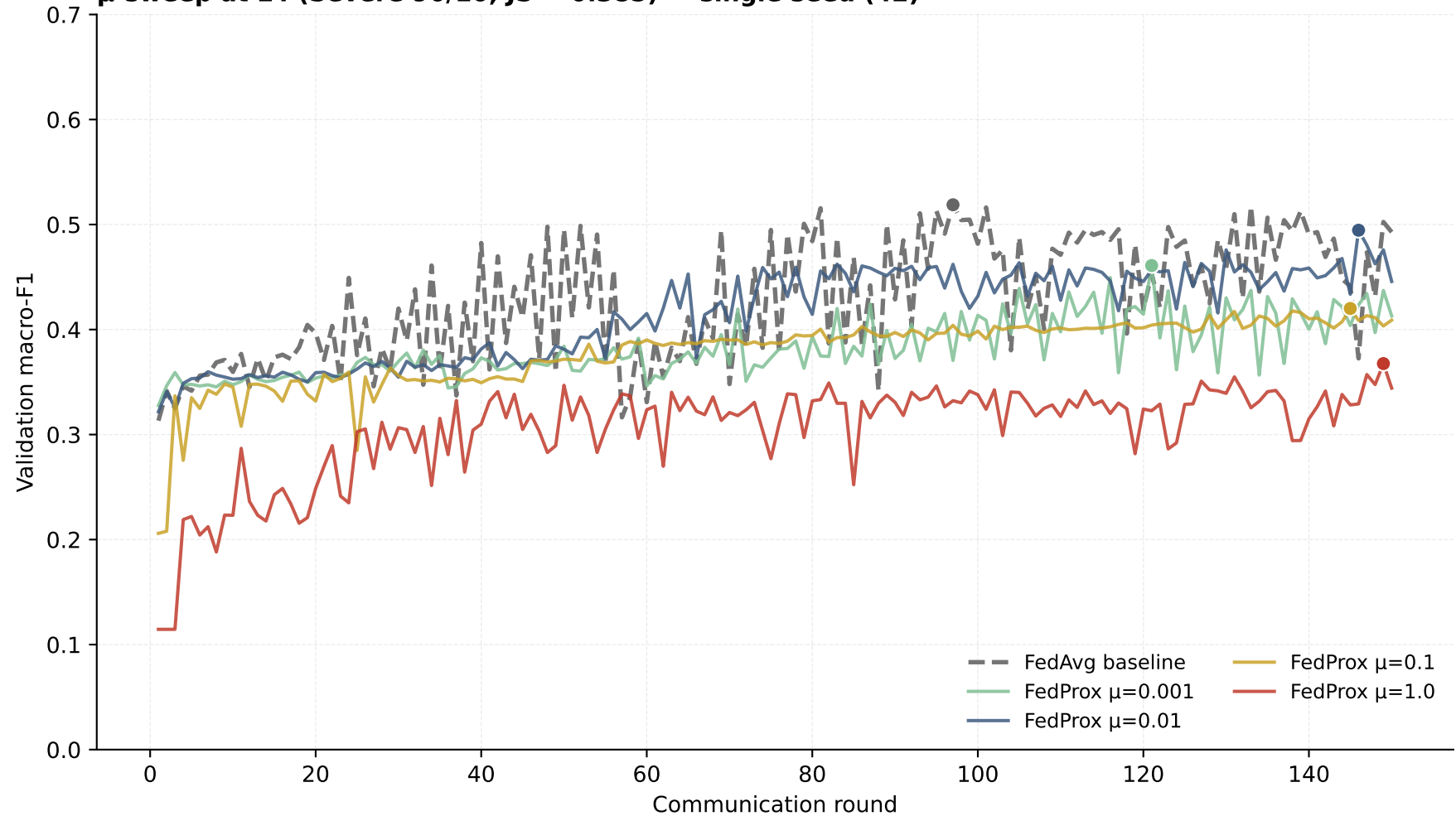
\mu -sweep at L4 (Severe 90/10, JS = 0.385) — single seed (42)
