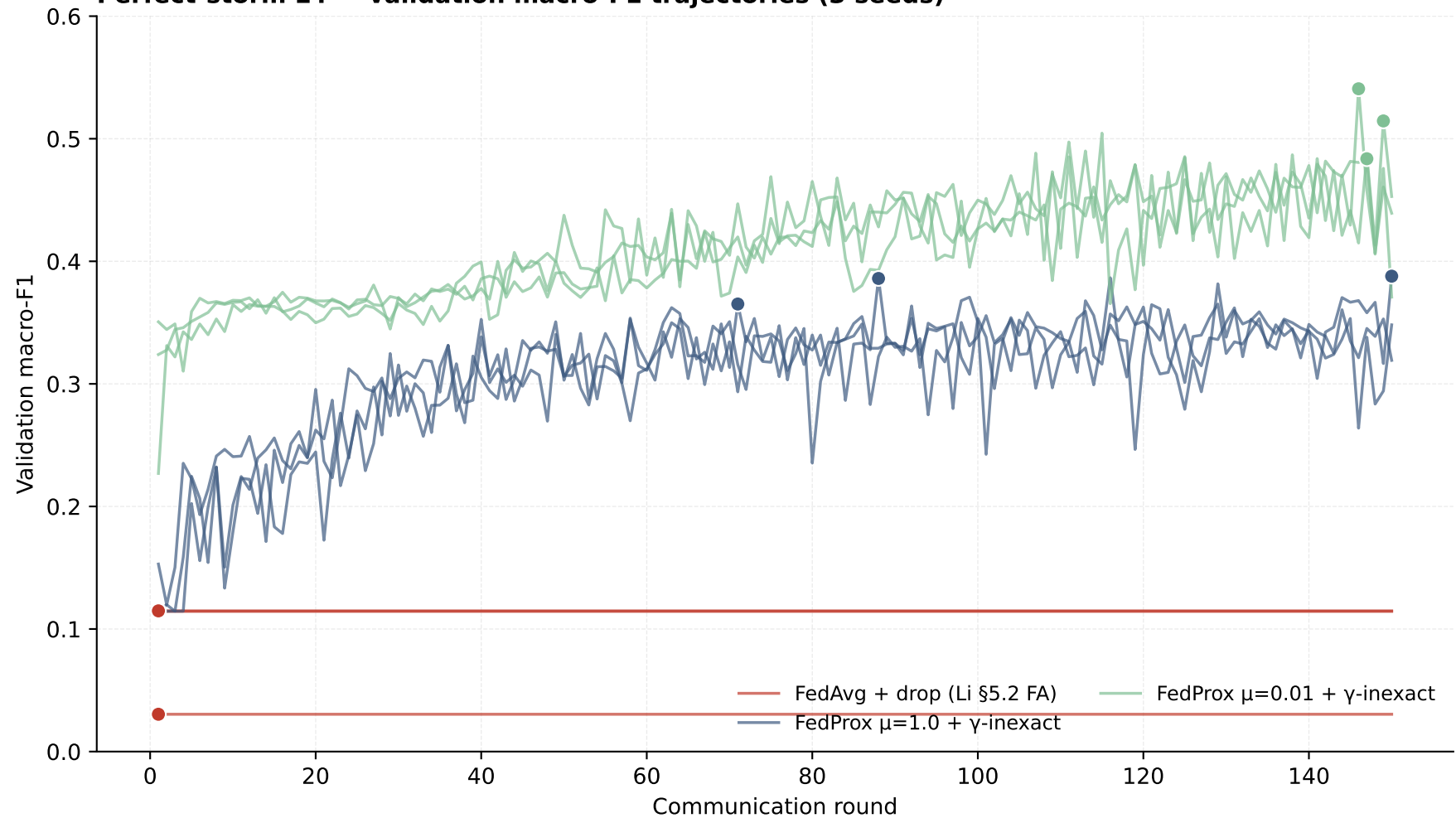
Perfect-storm L4 — validation macro-F1 trajectories (3 seeds)
