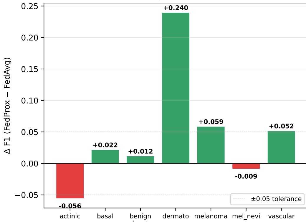
(F) Per-class \Delta (green = FedProx better)
