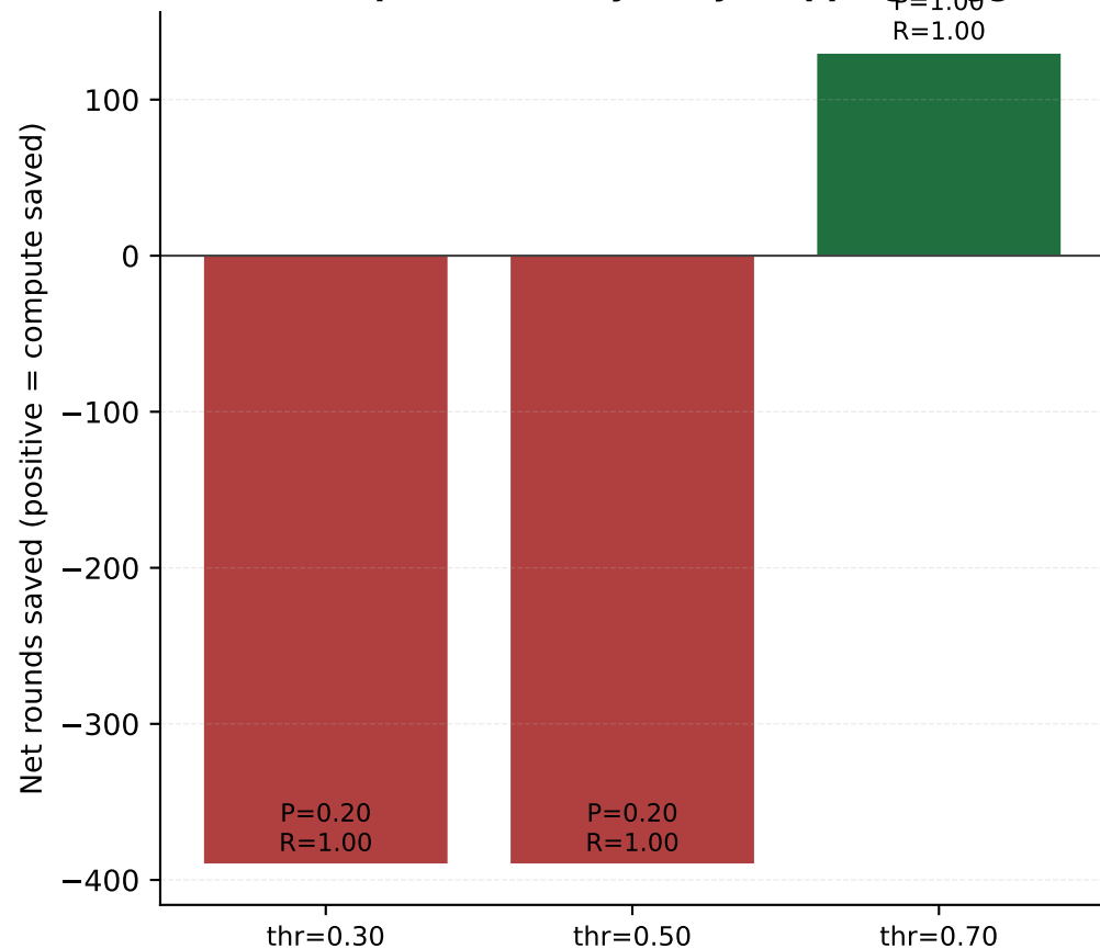
(b) Net compute saved by early-stopping flagged runs
