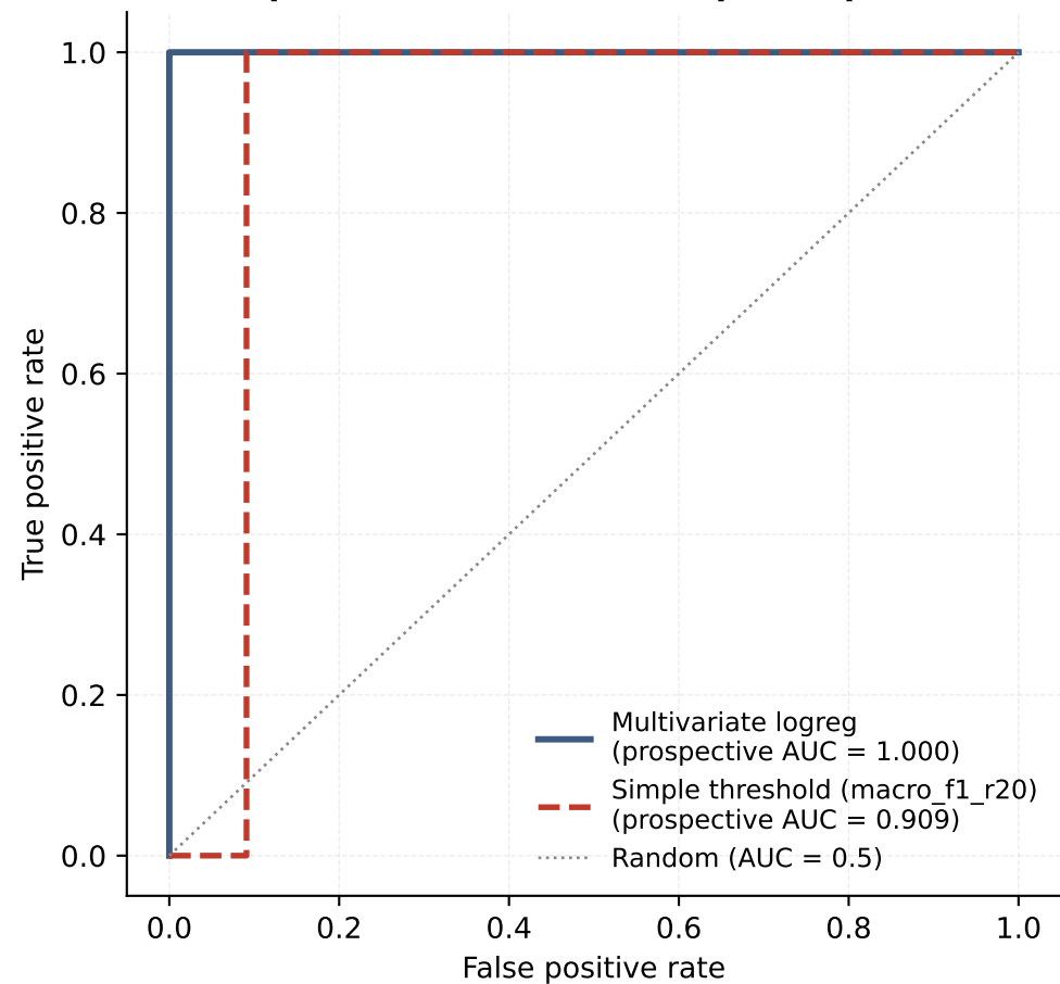
(a) Prospective ROC on held-out \mu -sweep (12 runs)
