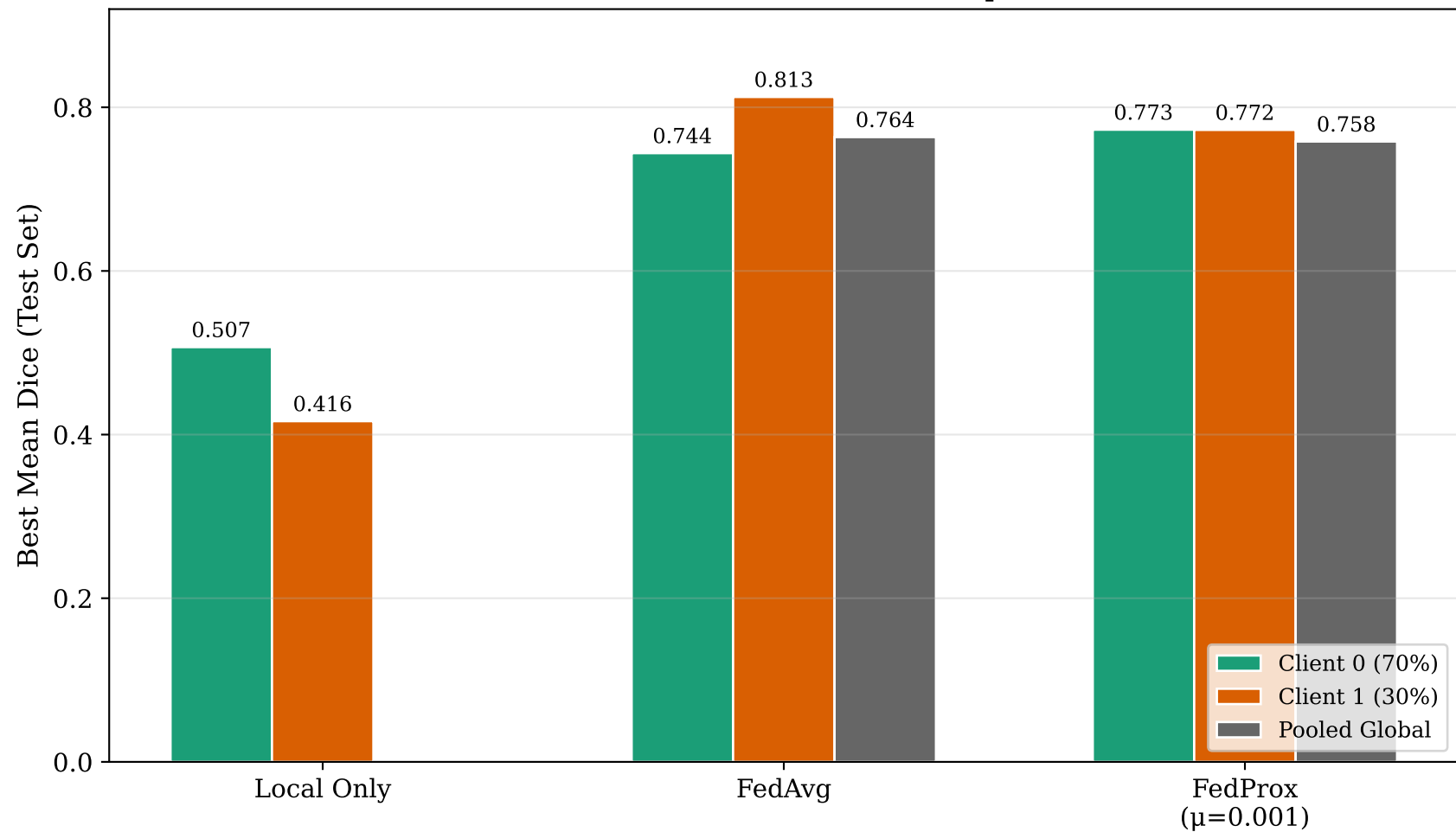
Federation Benefit: Best Mean Dice per Client
