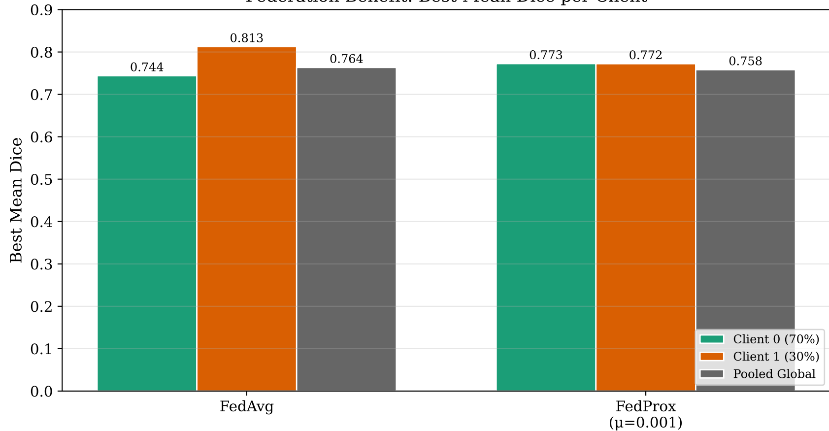
Federation Benefit: Best Mean Dice per Client
