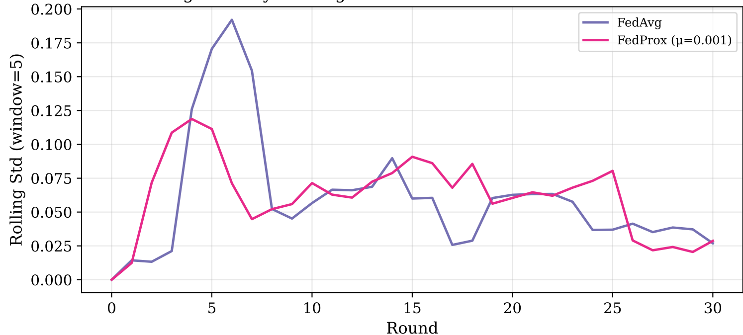
Training Stability: Rolling Standard Deviation of Global Mean Dice
