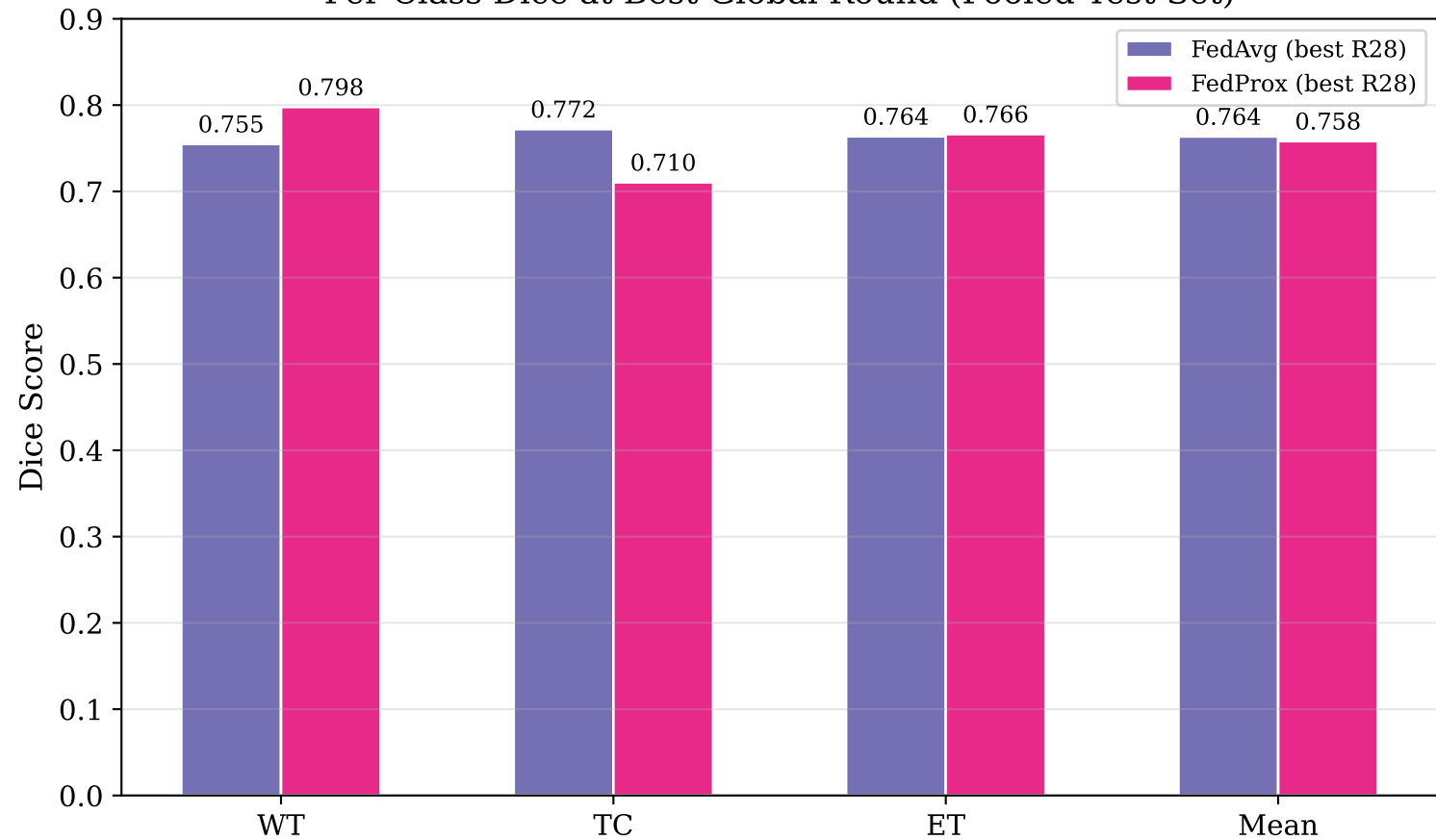
Per-Class Dice at Best Global Round (Pooled Test Set)
