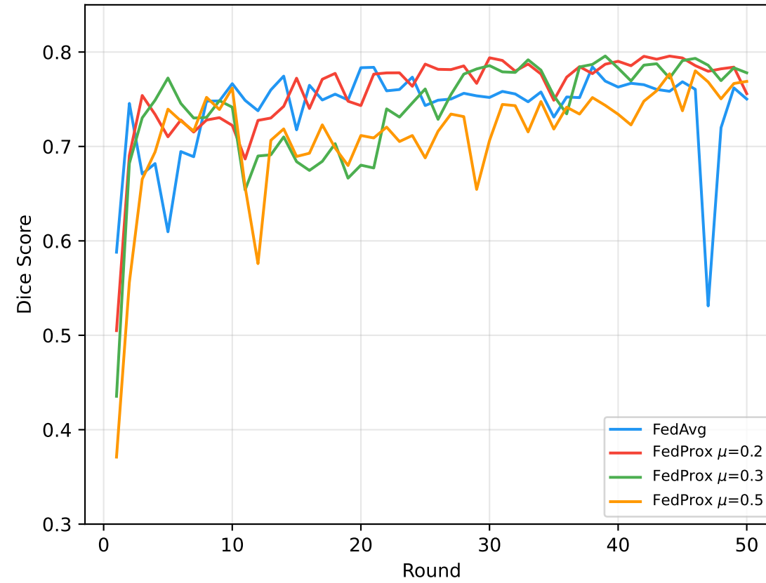
Global Dice vs \mu
