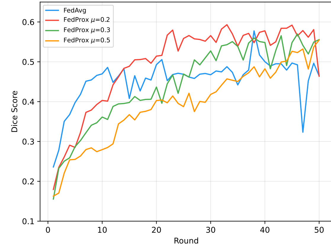
Client 1 (Corrupted) Dice vs \mu
