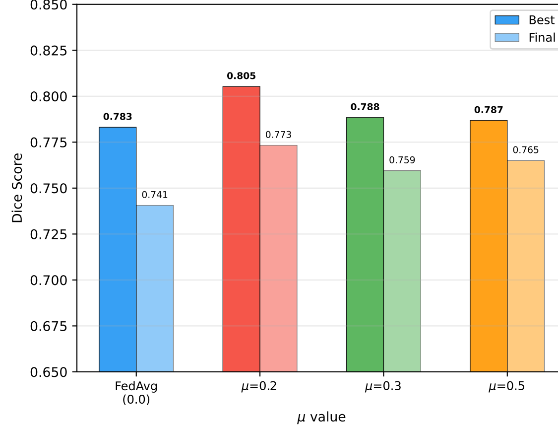
Global Dice vs \mu
