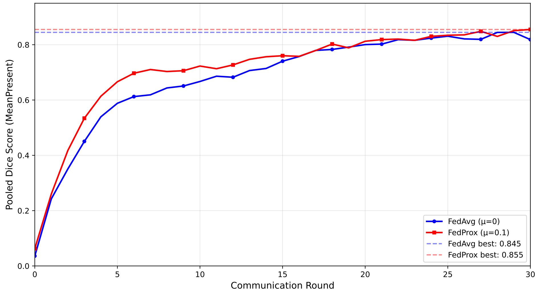
FedAvg vs FedProx: Global Model Convergence (BraTS 2D, 4 Clients, Dirichlet \alpha=1.0 )
