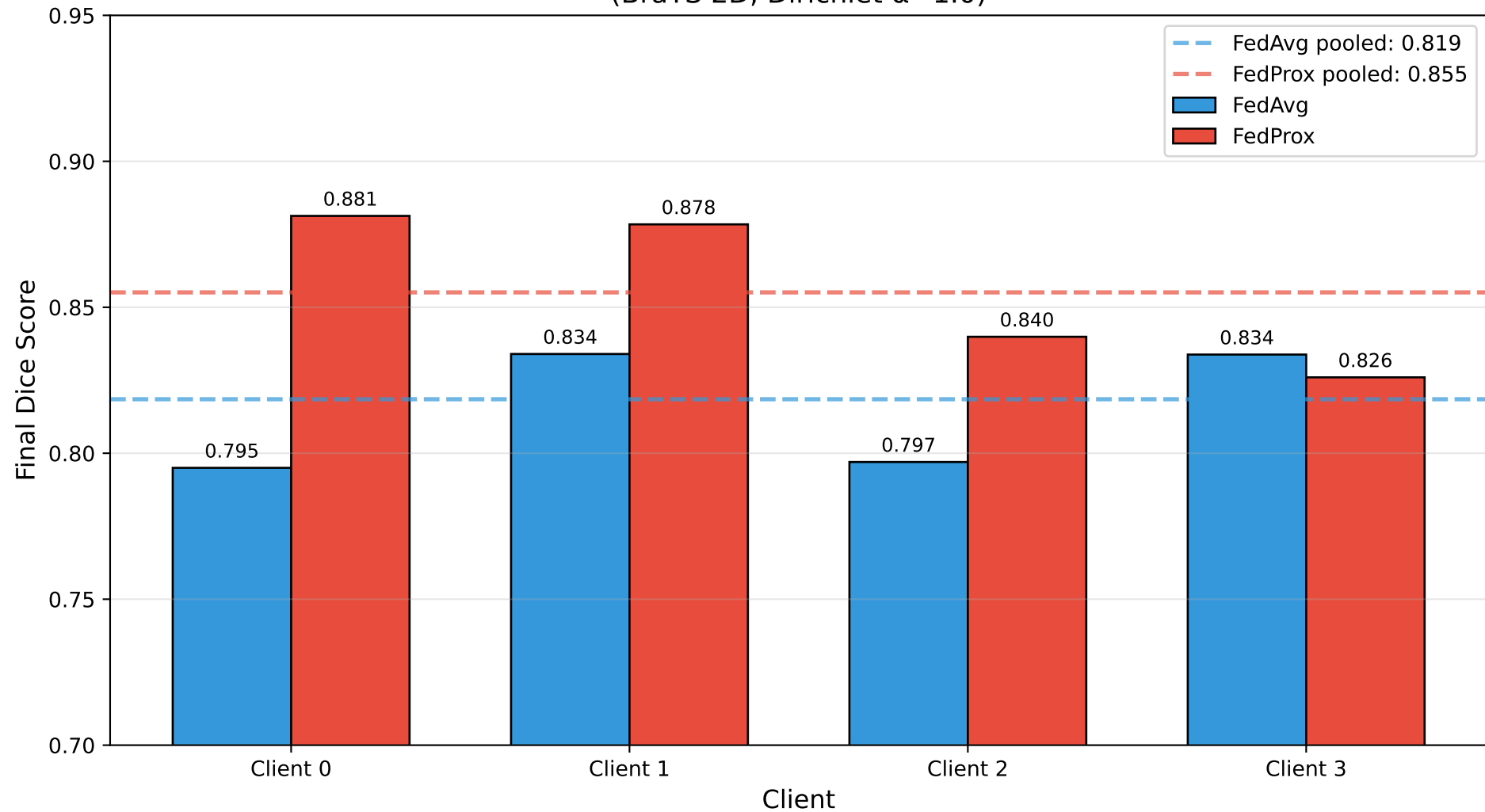
Final Round Per-Client Dice: FedAvg vs FedProx (BraTS 2D, Dirichlet \alpha=1.0 )
