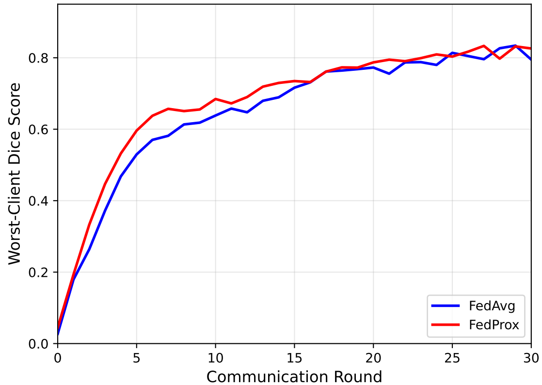
Worst-Client Performance (Fairness)
