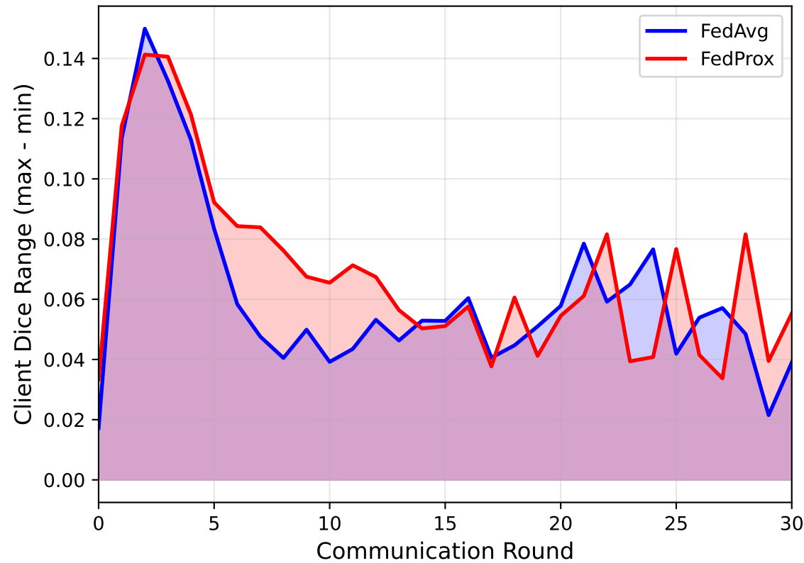
Client Performance Divergence
