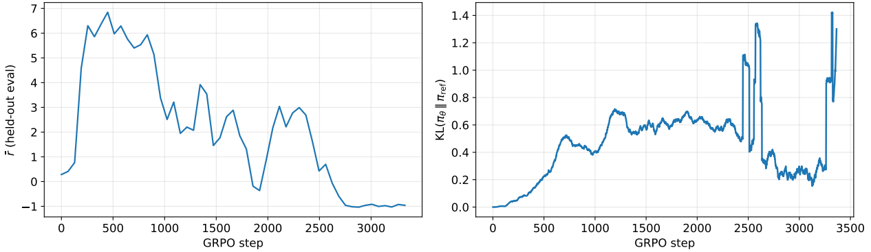
Figure 1: Baseline GRPO training vs. step (W&B run jgs4c6k1 ). Left: held-out eval reward \bar{r} (mean per-rollout total reward summed over the four reward terms, every 64 steps). Right: per-step reference-KL KL(\pi_\theta || \pi_{ref}) , 64-step moving average.
