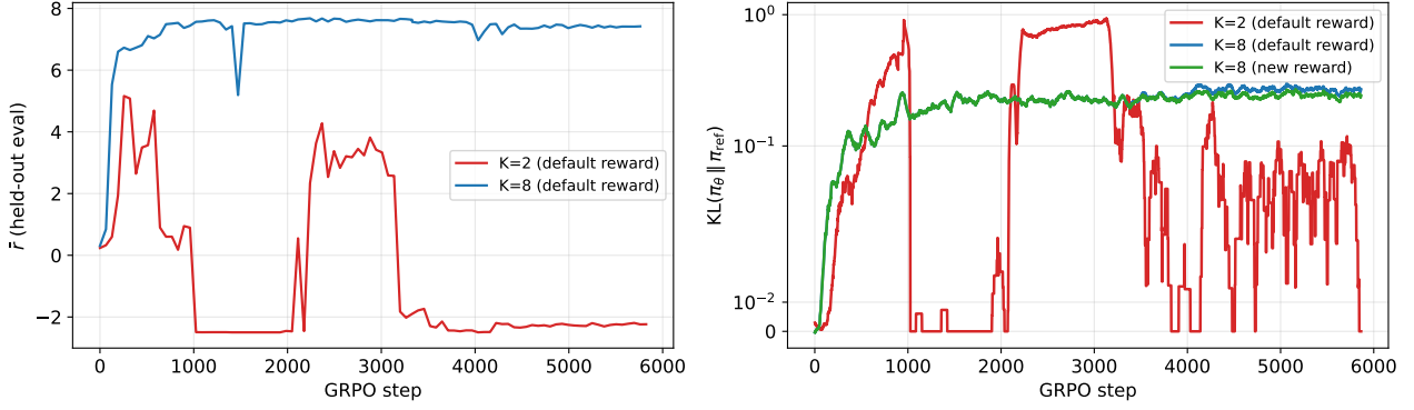
Figure 2: Training dynamics (held-out, every 64 steps). Left: eval reward \bar{r} (two default-reward runs). Right: reference-KL KL(\pi_\theta || \pi_{ref}) for all three runs (64-step moving average, symlog y -axis).
