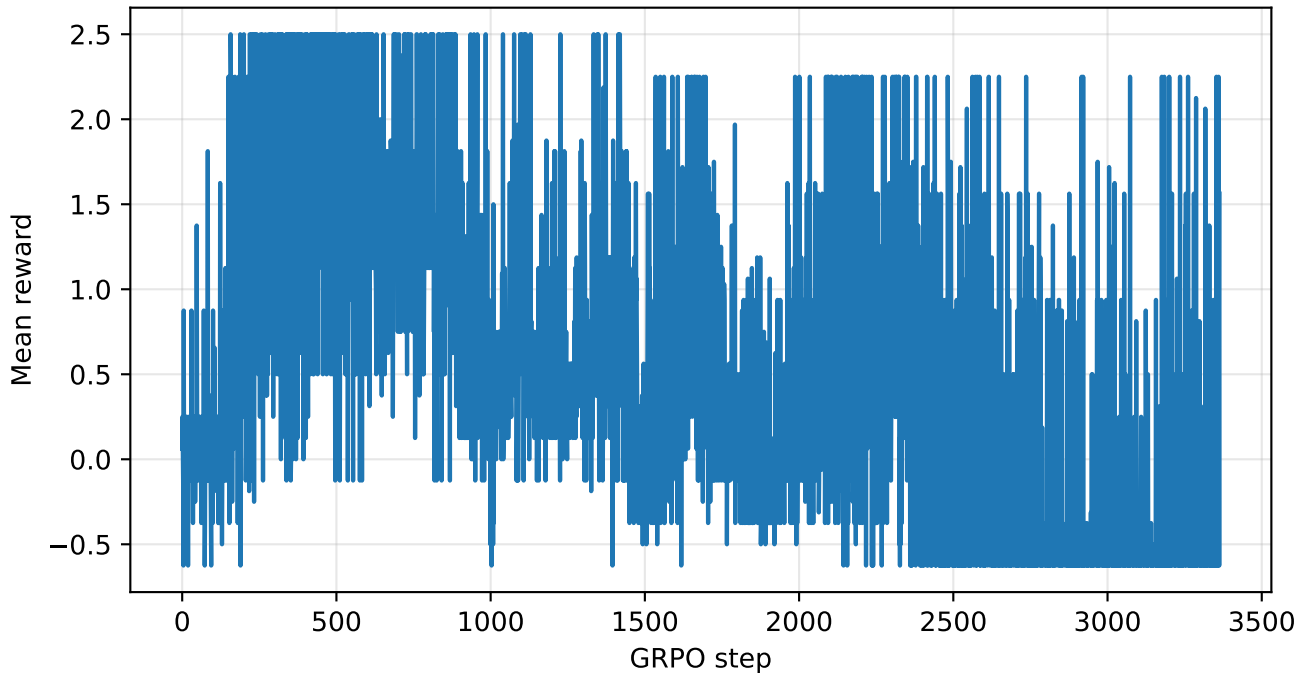
Baseline GRPO training reward
