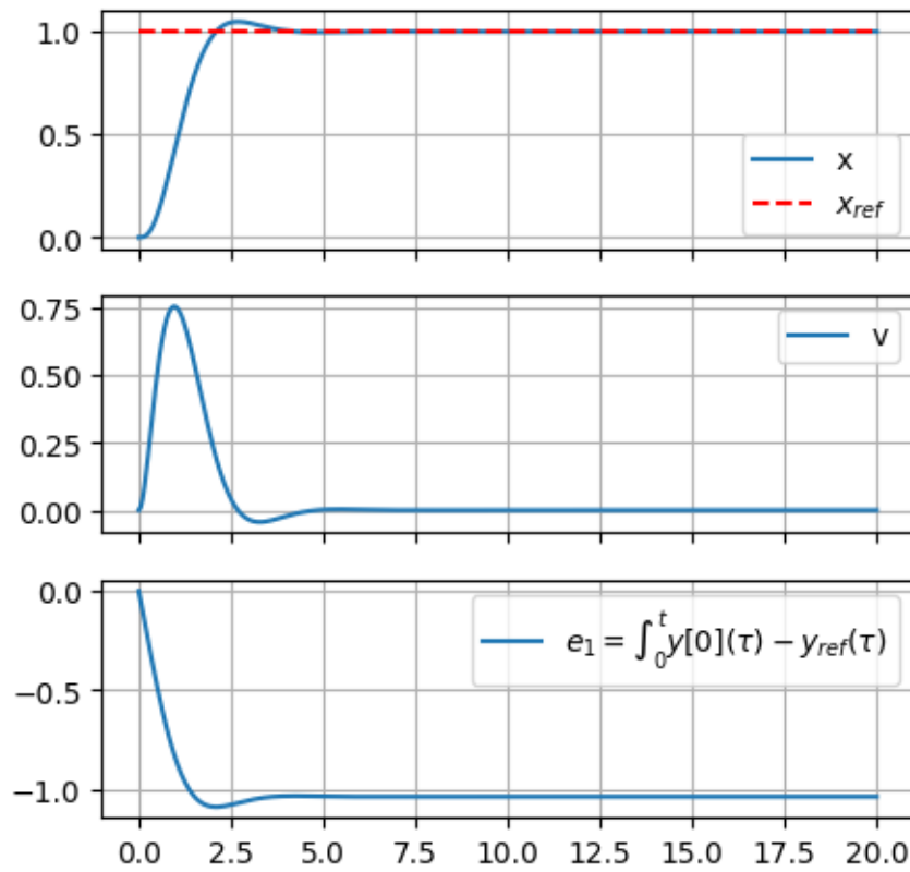
Step response
