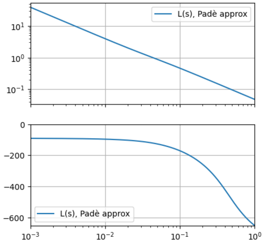
Bode plot of L(s)
