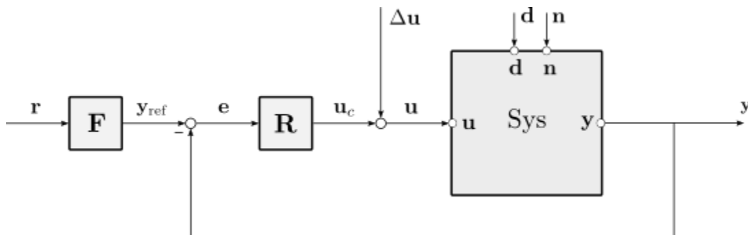
Fig. 44.1: Block diagram of the closed-loop system
