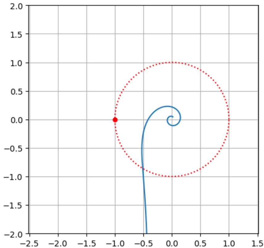
Nyquist diagram of L(s)
