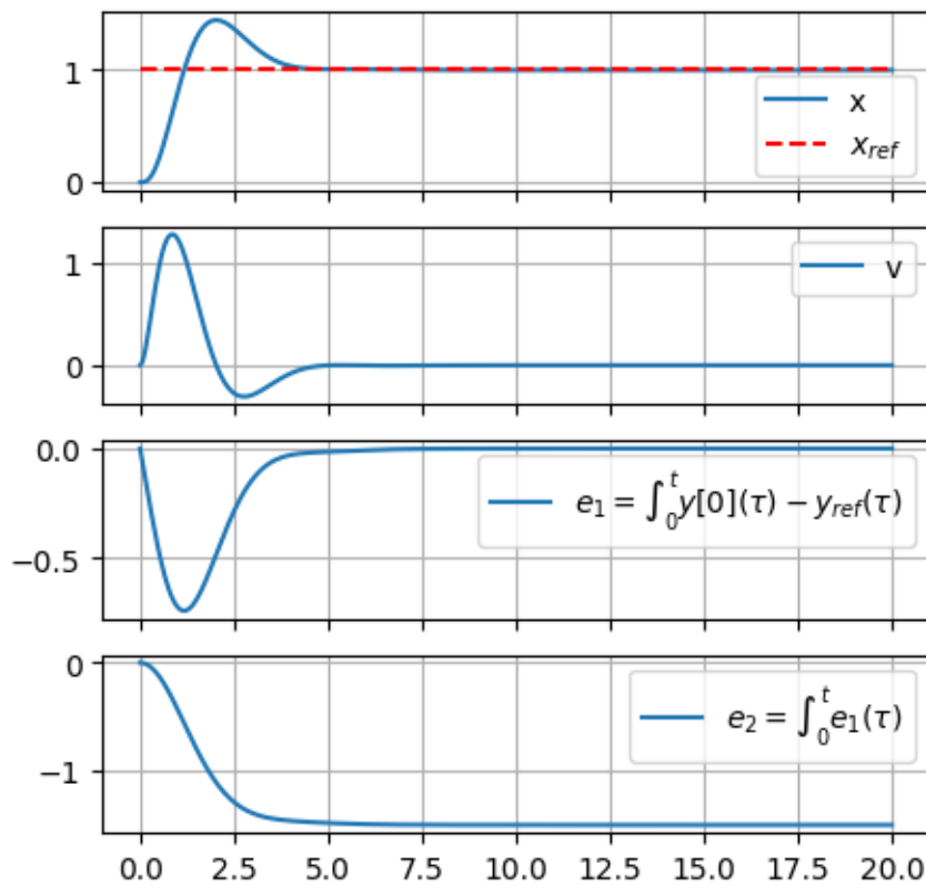
Step response
