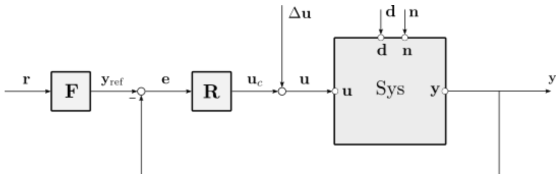
Fig. 41.1: Block diagram of the closed-loop system
