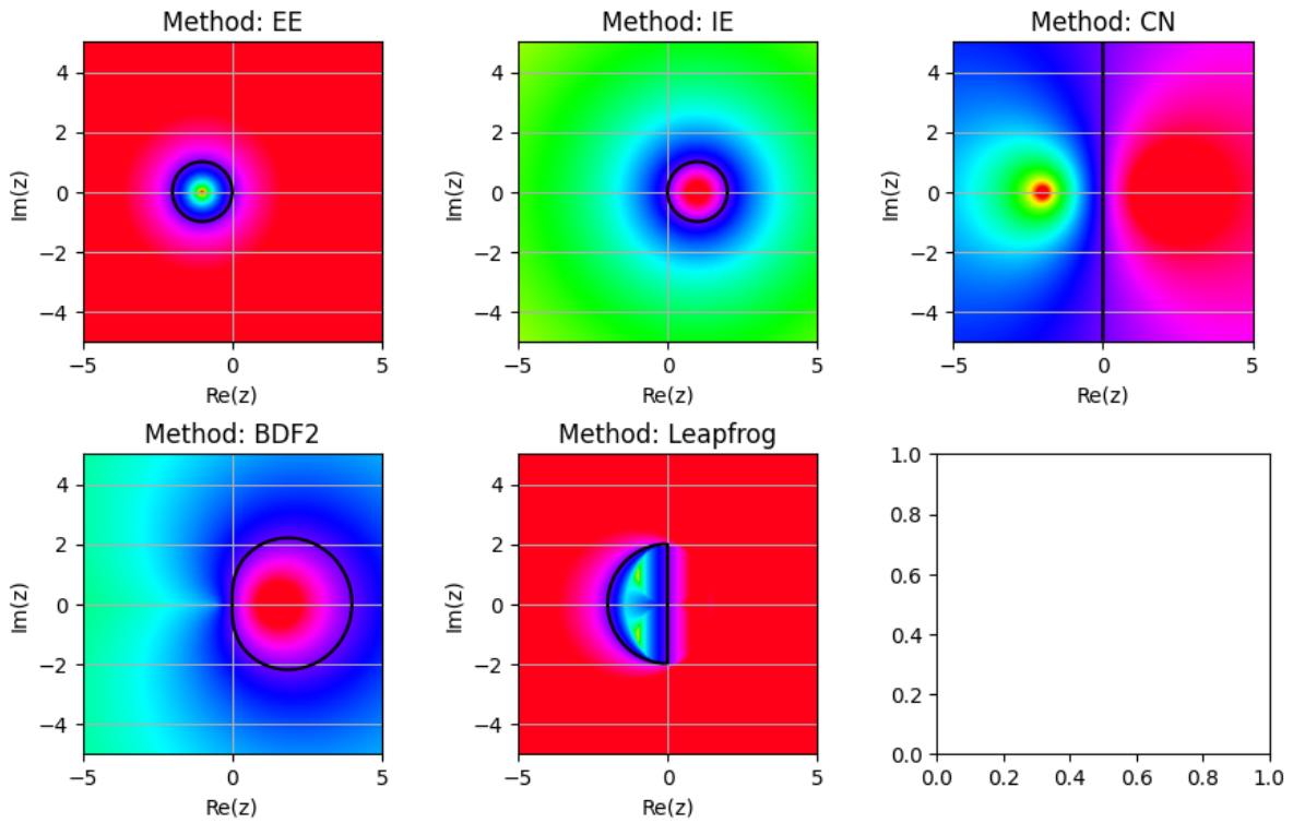
Magnitude of one-step TF, |G(z)|
