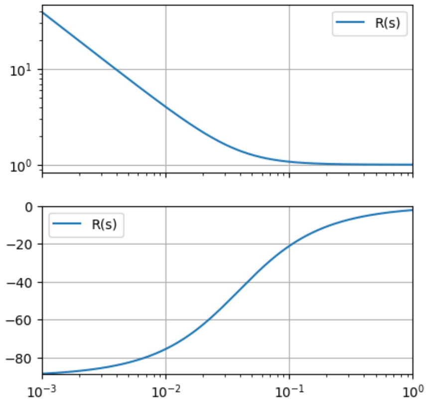
Bode plots of the PI controller
