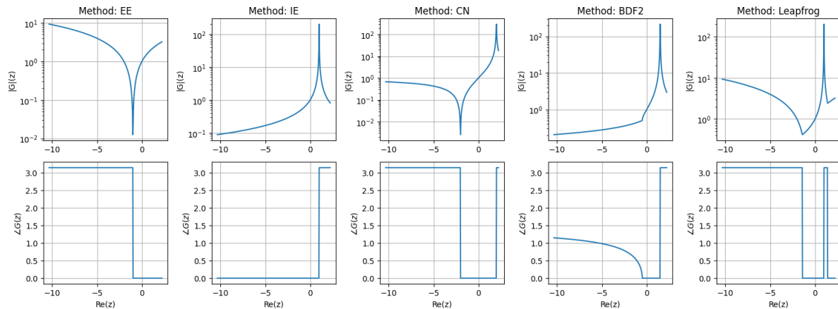
One-step TF on the real axis, G(z), z \in \mathbb{R} .
