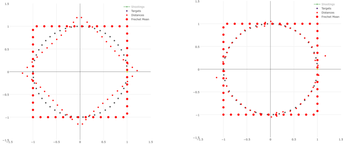
(a) Kernel scale \sigma = 2
