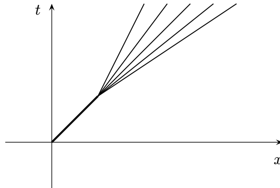
Figure 4: A discontinuity diverging into multiple characteristics
