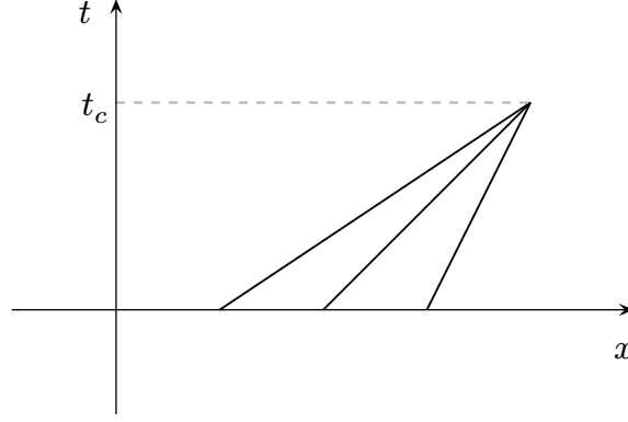
Figure 2: Crossing of characteristic curves.
