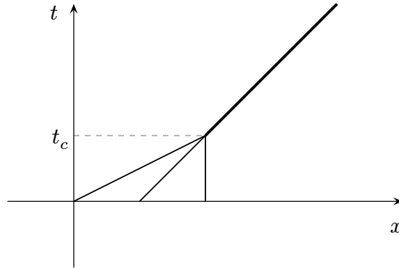
Figure 3: Creation of a shock
