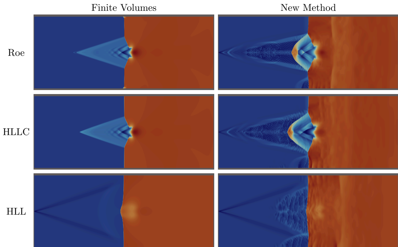
Figure 13: Todo
