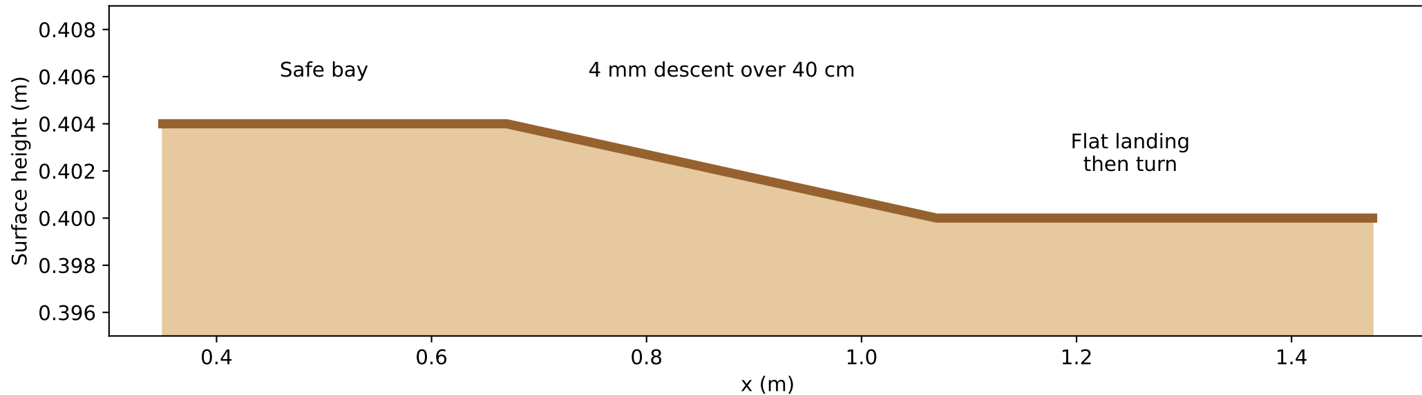
Side profile through the first leg (vertical scale exaggerated)
