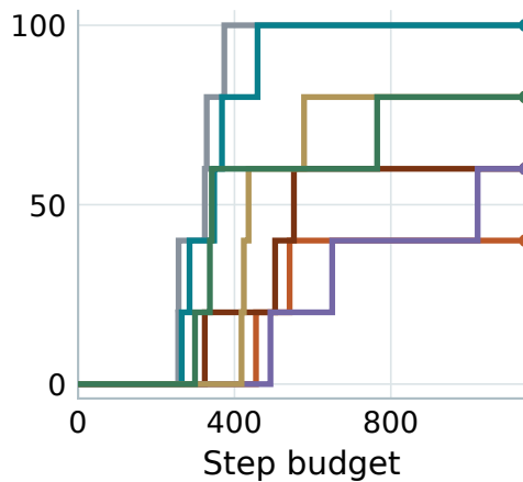
Runs solved (%)
