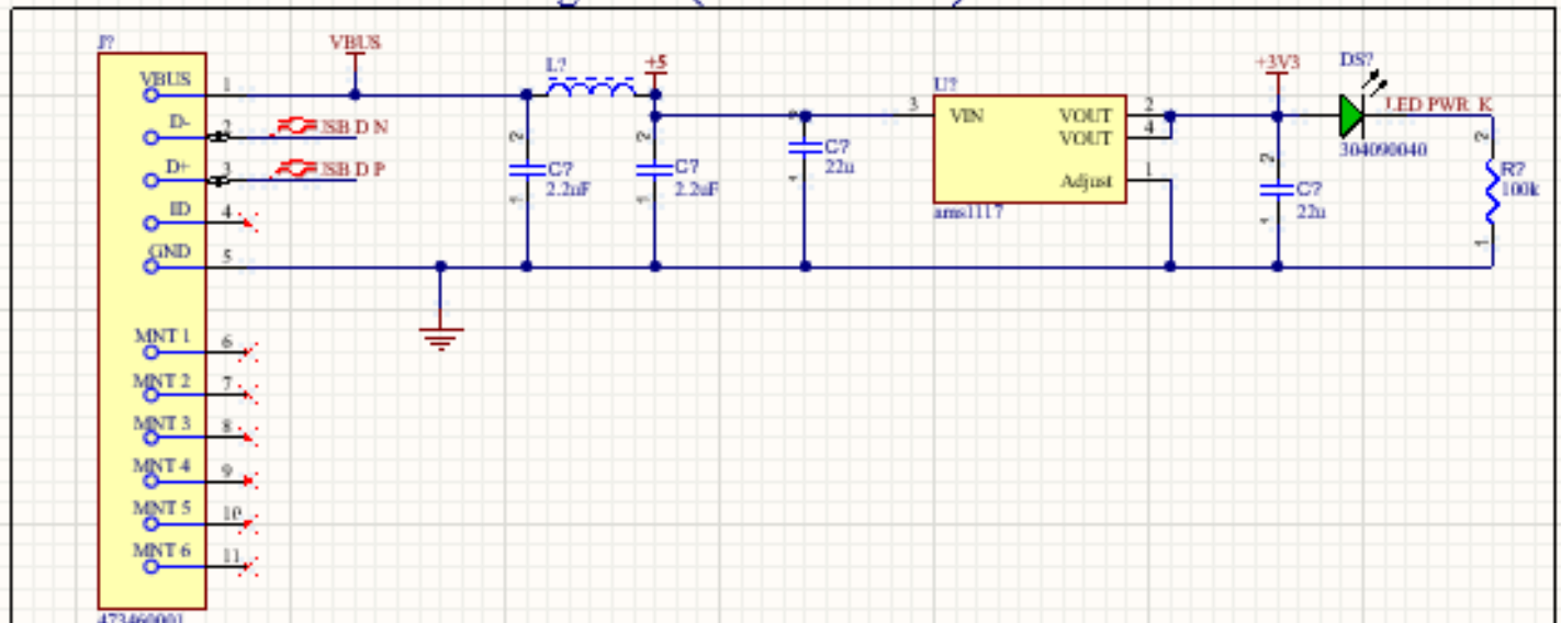
USB Connector and LDO Regulator(+5V to +3V3)
