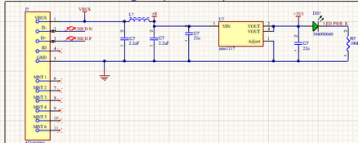
USB Connector and LDO Regulator(+5V to +3V3)
