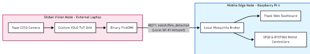
Figure 4. 1: High-level system architecture detailing the physical and logical decoupling of the external Global Vision Node and the Raspberry Pi 4 Mobile Edge Node.
