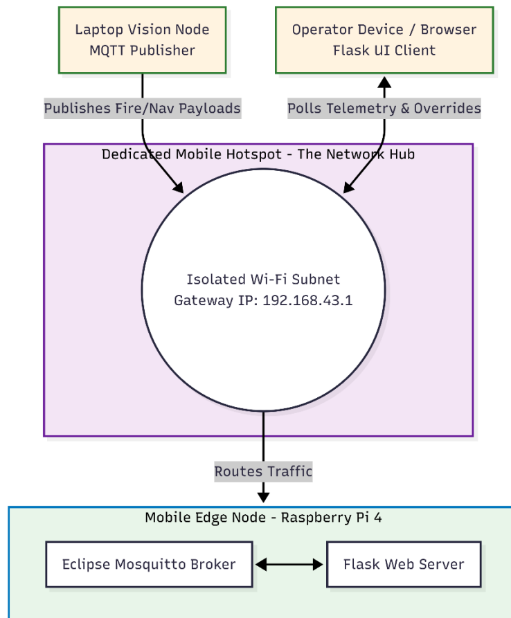
Figure 4. 2: Network topology demonstrating the flow of asynchronous MQTT payloads and video telemetry through a dedicated Mobile Hotspot, ensuring zero external network dependency for the Project Phoenix integration layer.
