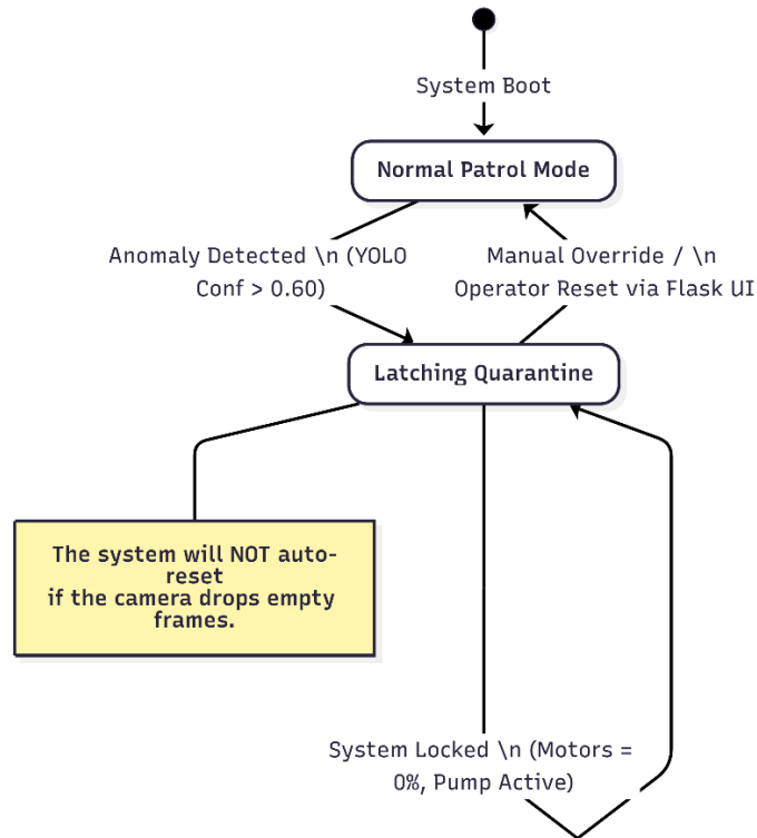
Figure 8. 1: State machine diagram illustrating the software-enforced latching quarantine logic. The system deliberately requires a manual operator reset via the Flask dashboard to ensure human verification of the suppressed hazard.
