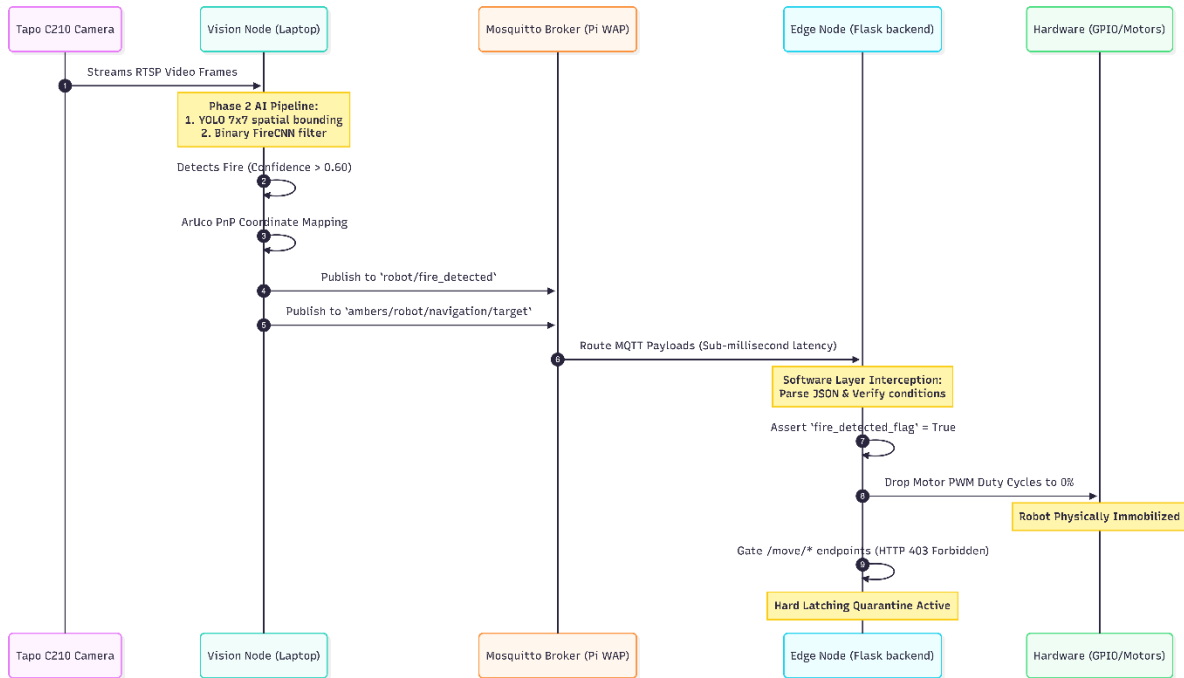
Figure 9. 1: UML sequence diagram mapping the deterministic chronological event chain of the AI-to-Control integration pipeline, from initial Phase 2 AI perception to localized hardware motor suppression.
