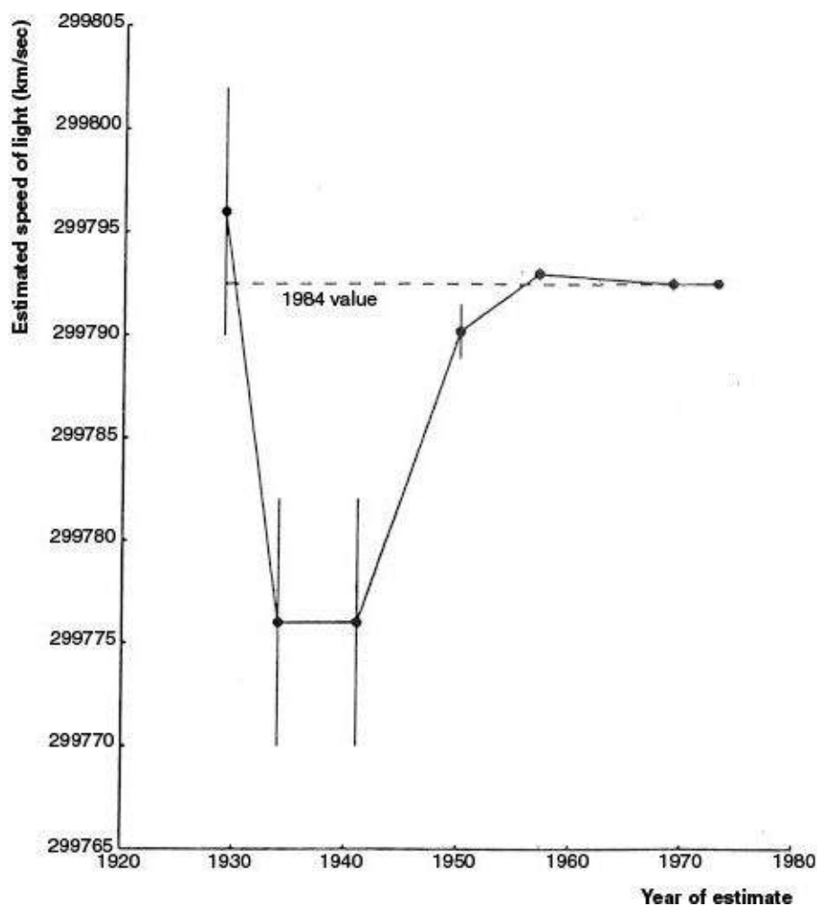
Figure 37.2. Recommended values for the velocity of light; 1929–1973.
