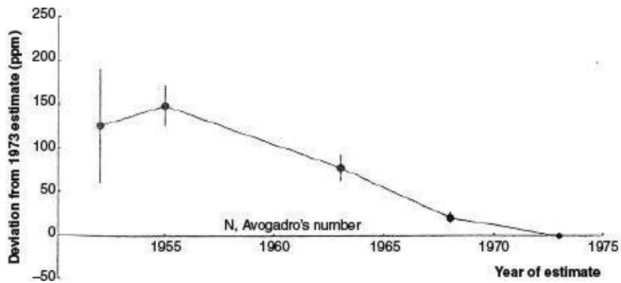
Figure 37.3. Recommended values for fundamental constants; 1952–1973.
