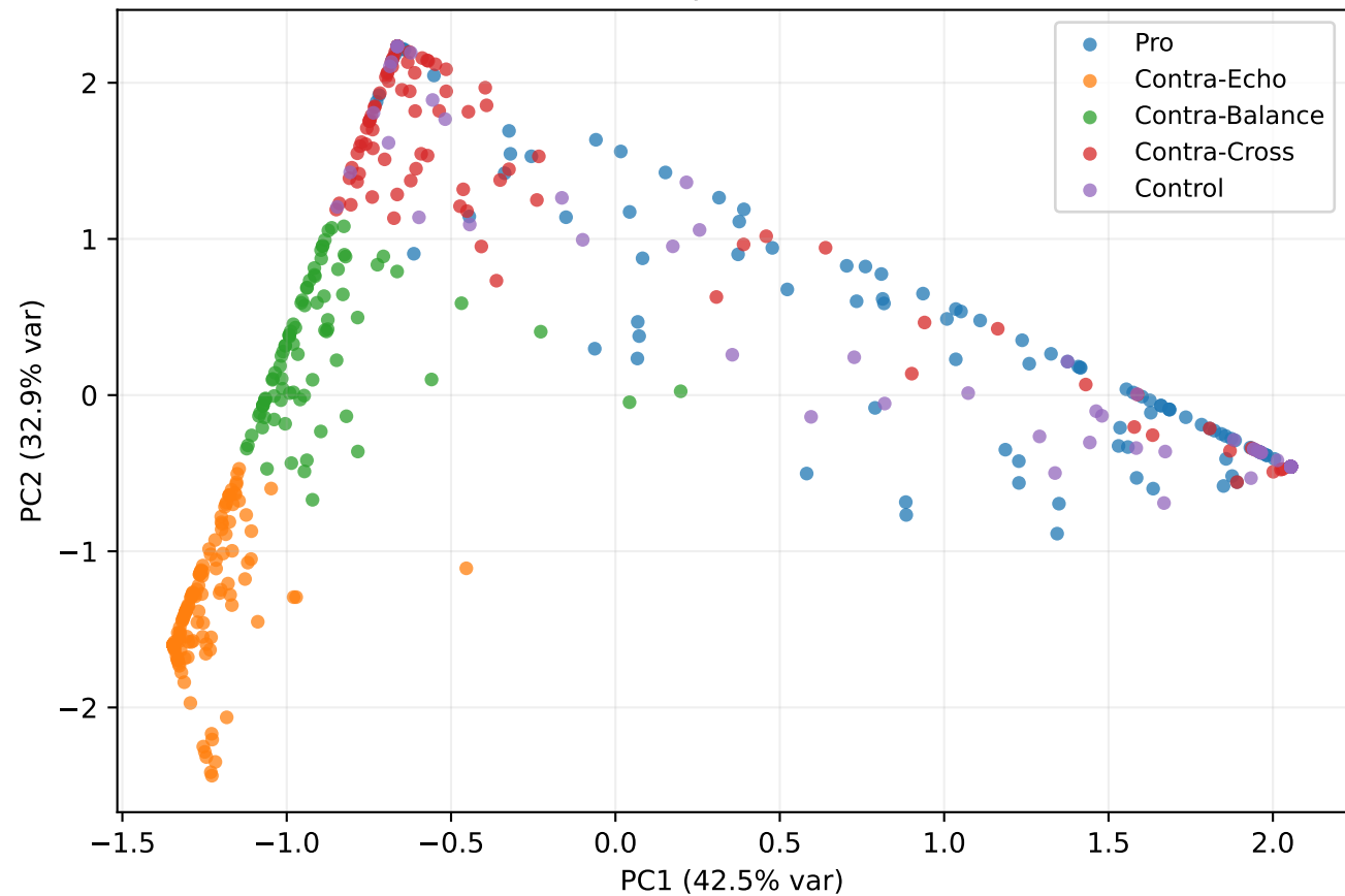
PCA of Interactional-Space Features (User-Level)
