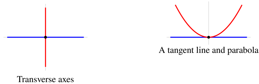
Figure 1.1: Two intersections with the same underlying set.
