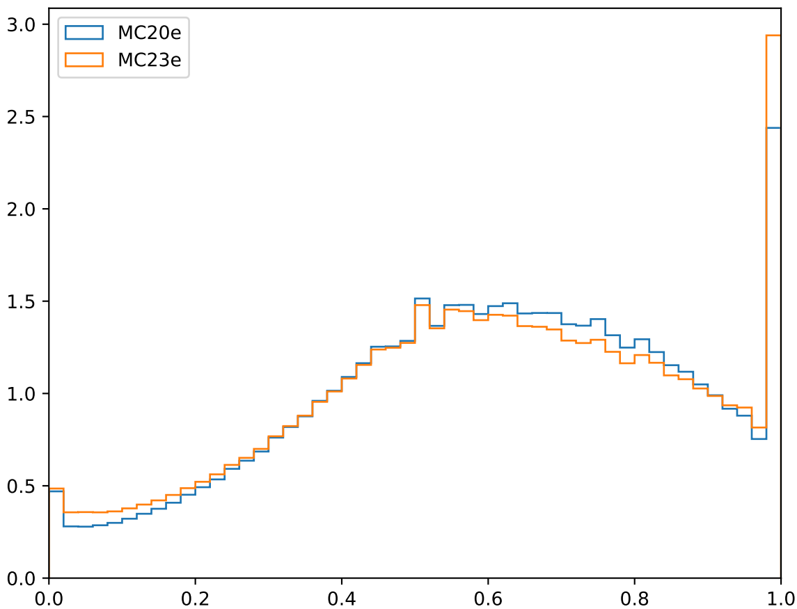
Relative number of clusters
