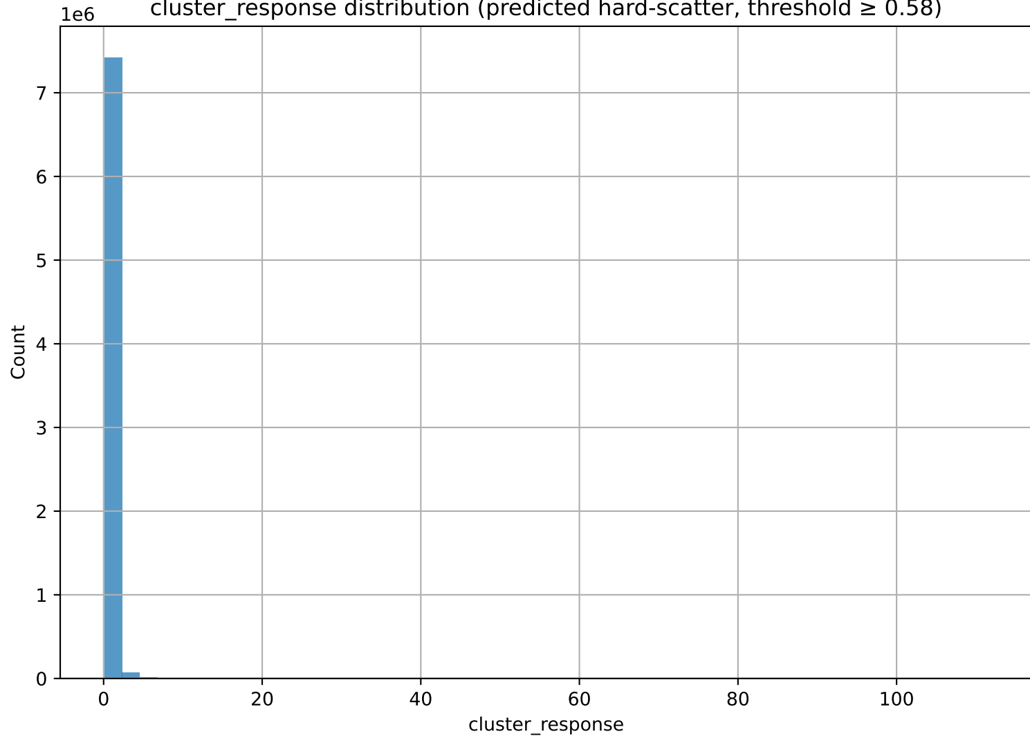
cluster_response distribution (predicted hard-scatter, threshold \geq 0.58 )
