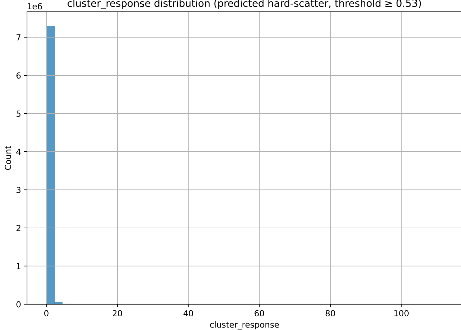
cluster_response distribution (predicted hard-scatter, threshold \geq 0.53 )
