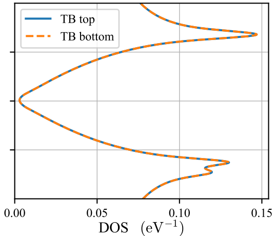
DOS (normalized)
