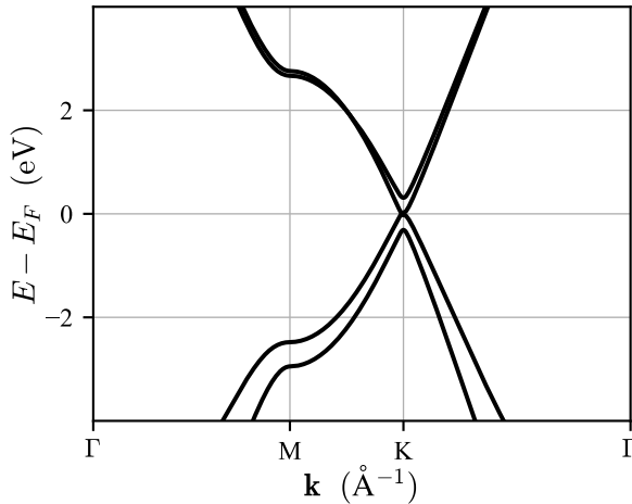
Band structure
