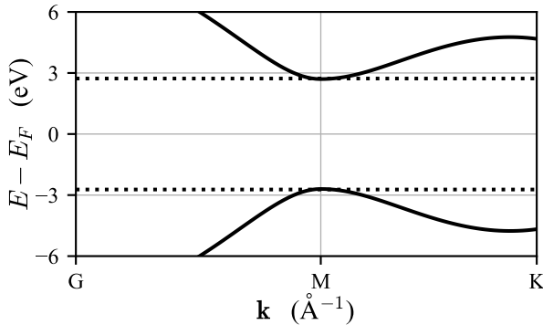
Band Structure
