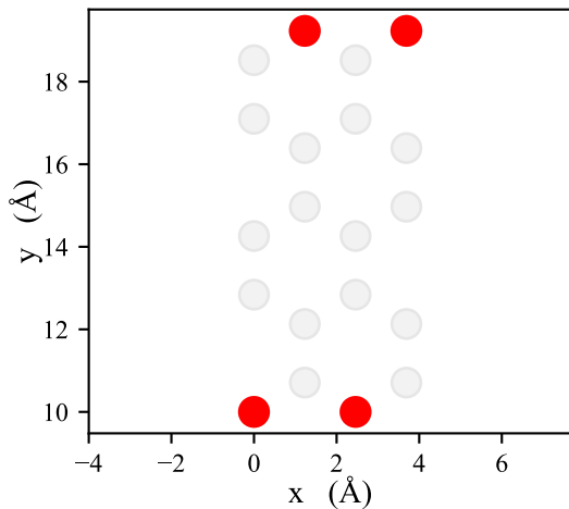
z-GNR, E=0.0 eV
