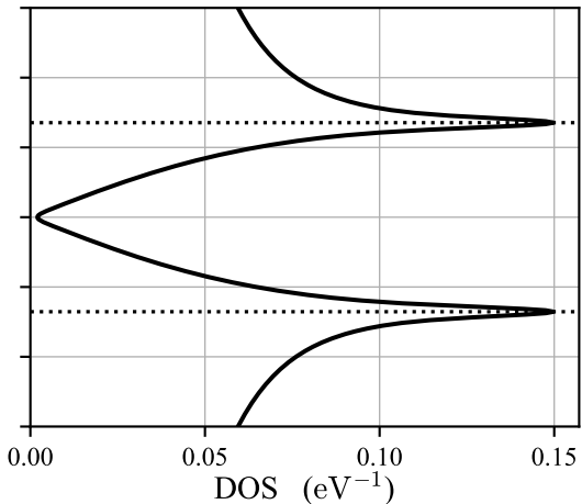
DOS (normalized)
