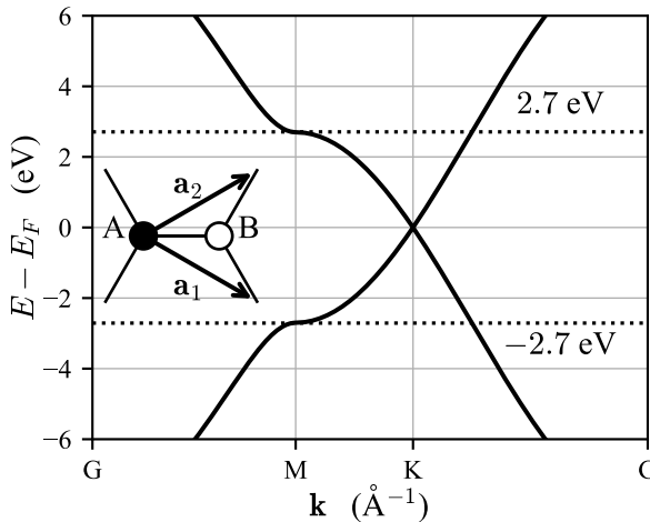
Band Structure
