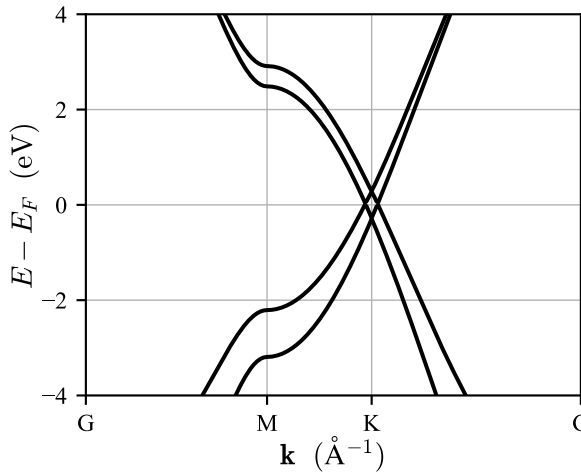
Band structure
