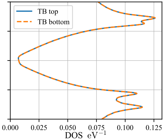
DOS (normalized)
