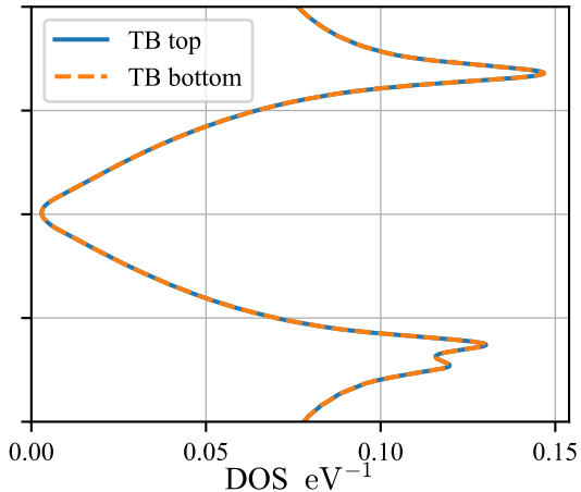
DOS (normalized)
